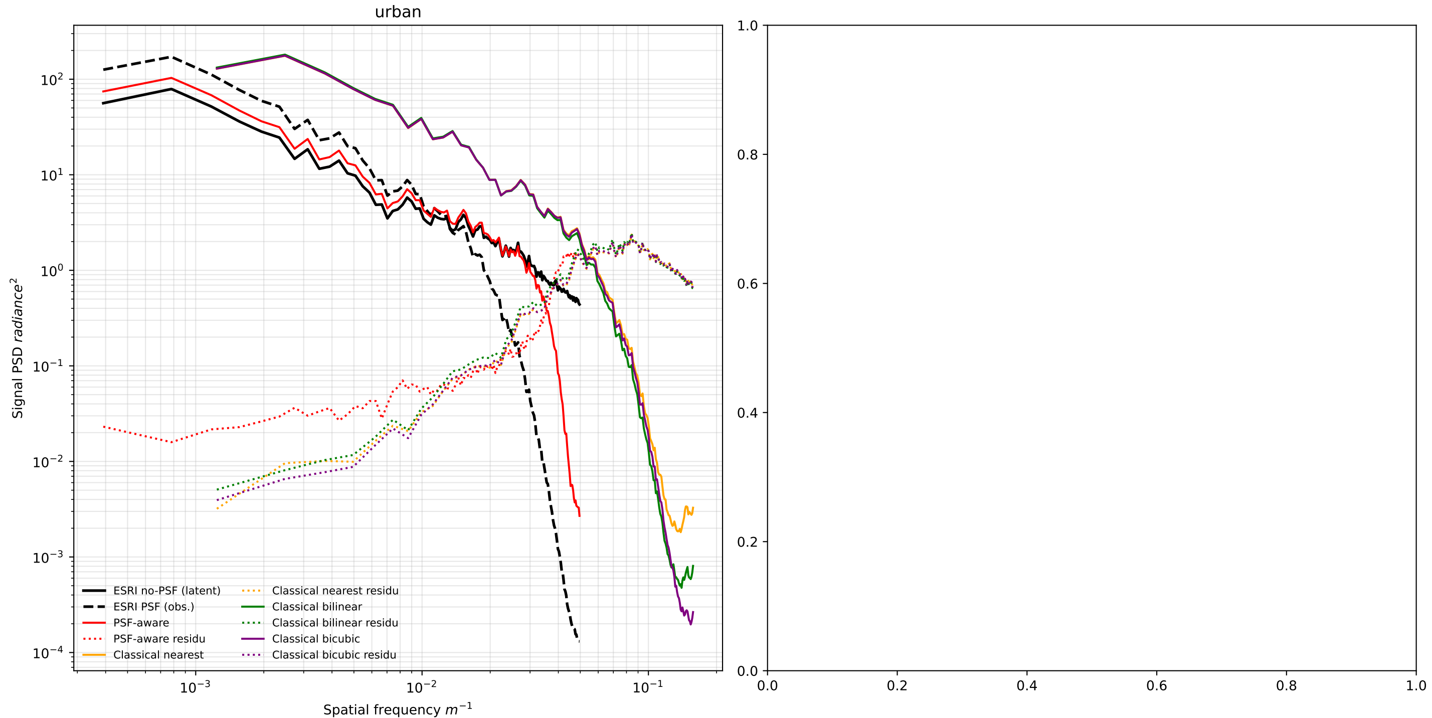
Synthetic detector 1D power spectra — all methods
