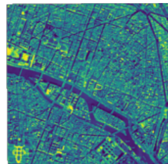
PSF-aware
