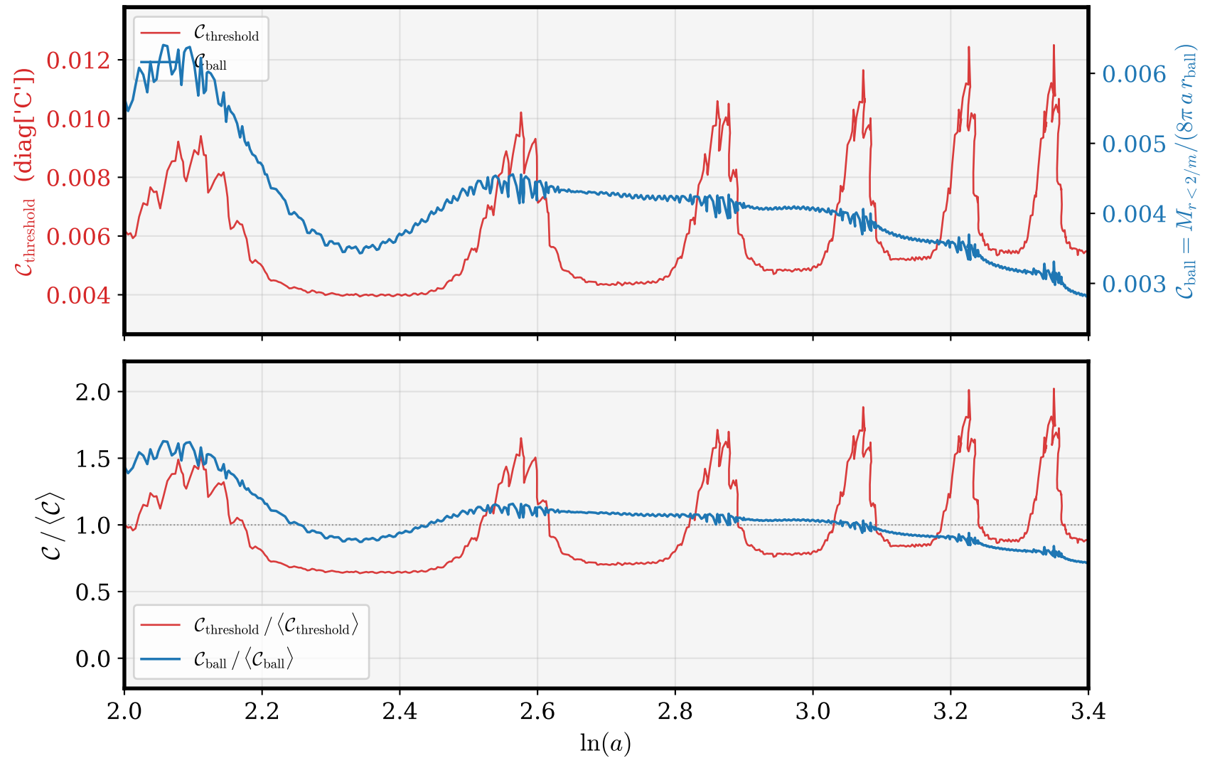
MR compactness: threshold-based vs coord.-ball ( \lambda_{\text{GB}} = 0 , g_2 = 10 , \Delta r = 1/24 )
