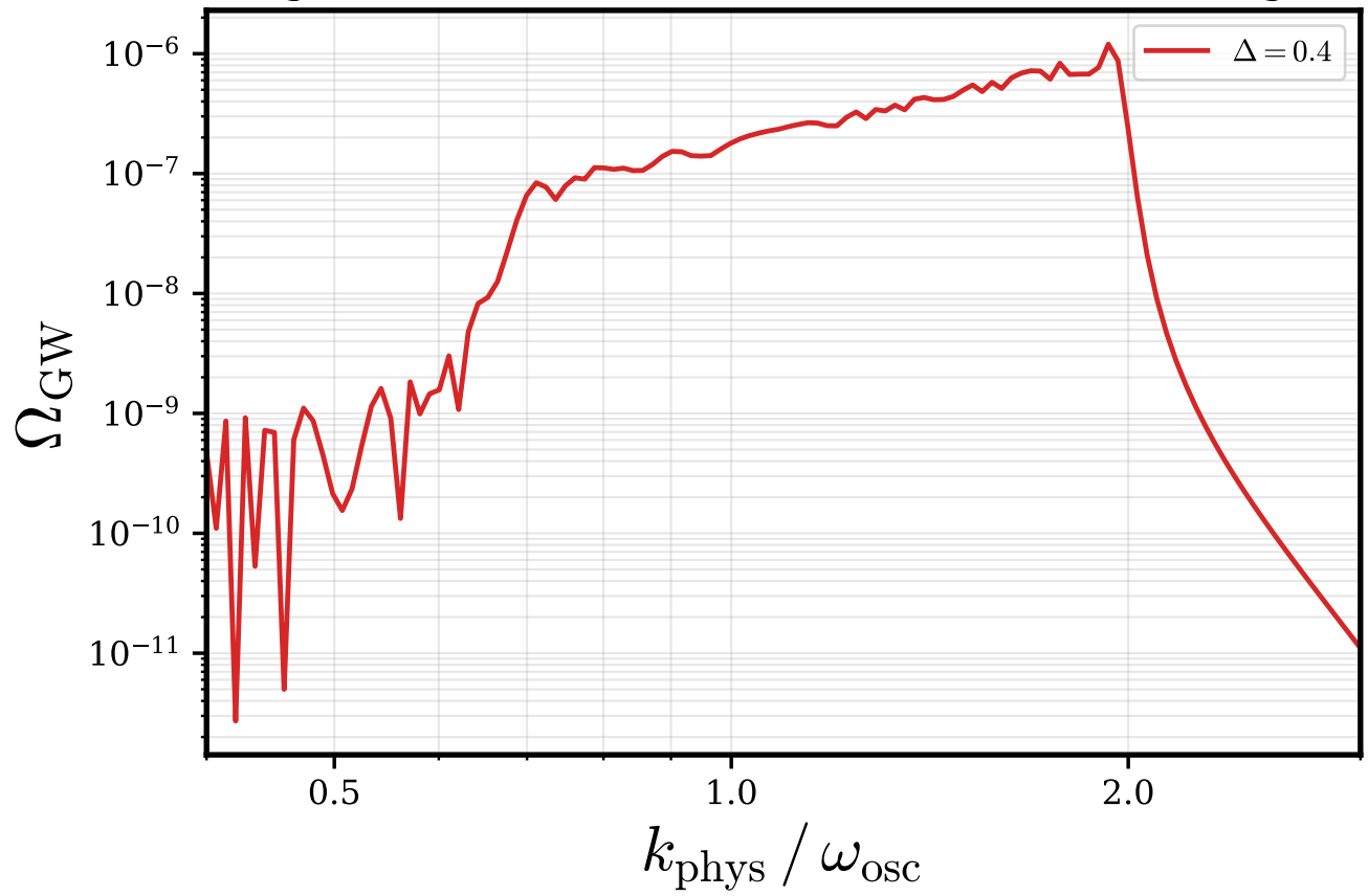
Benchmark of Fig. 2 (Antusch-Cefala-Orani 2017): w=0 , single oscillon, a_f=3
