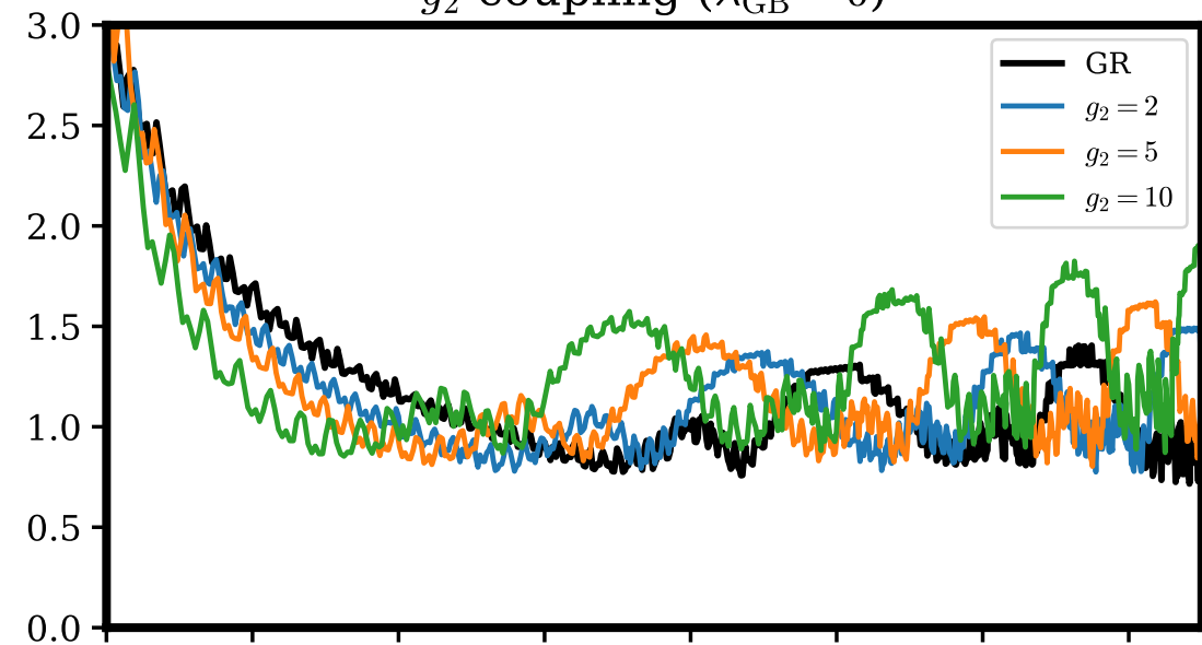
g_2 coupling ( \lambda_{\text{GB}} = 0 )
