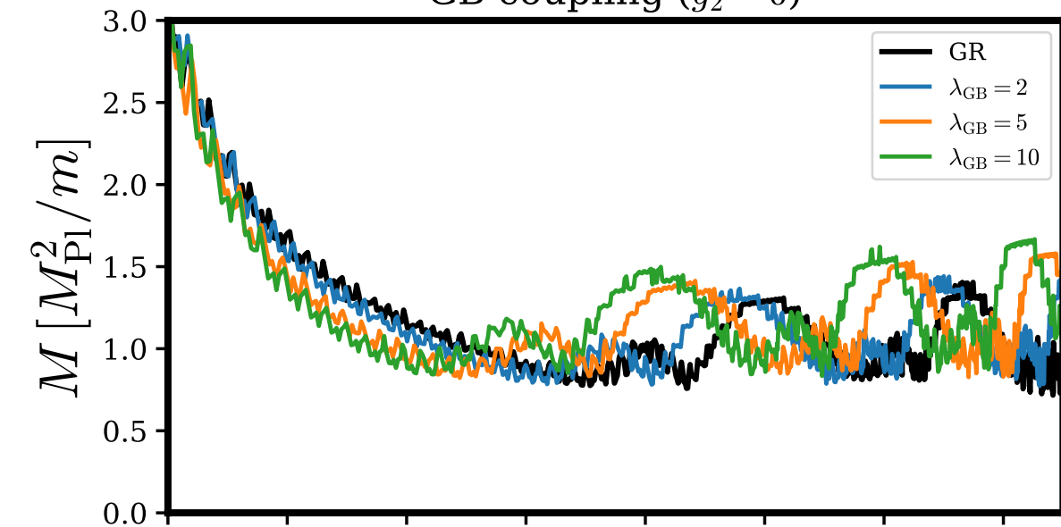
GB coupling ( g_2 = 0 )
