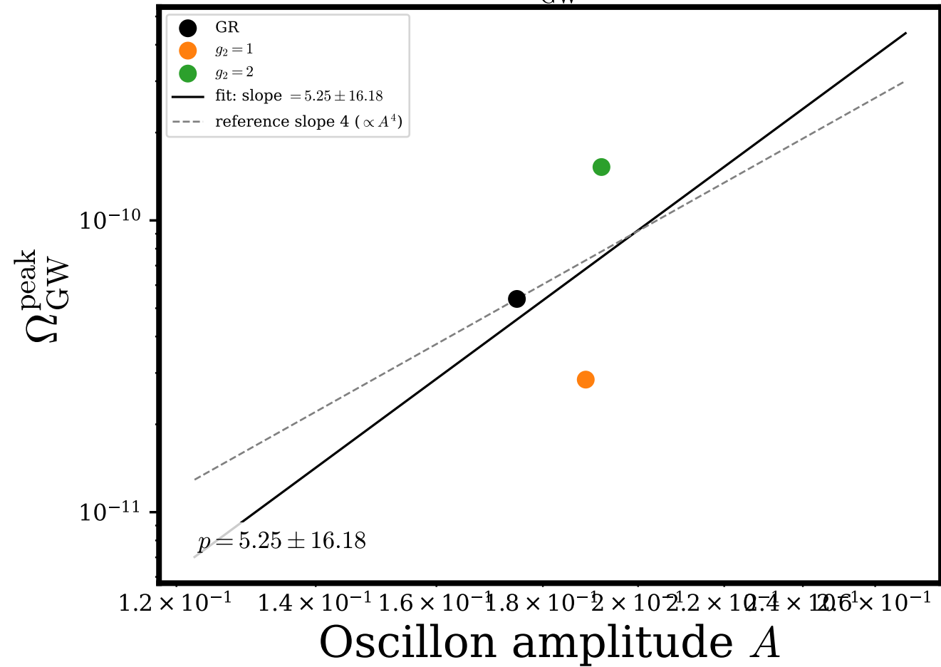
Raw \Omega_{\text{GW}}^{\text{peak}} vs A
