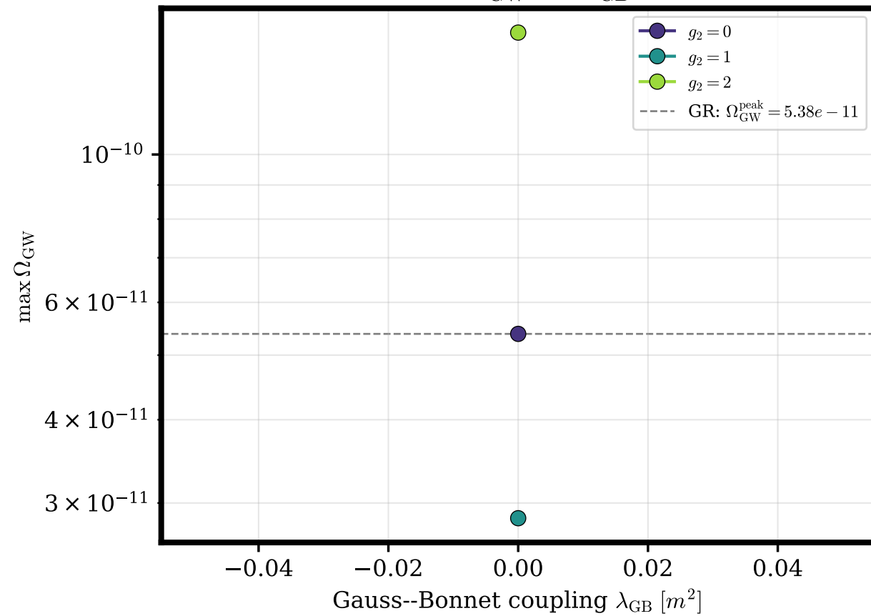
\max \Omega_{\text{GW}} vs \lambda_{\text{GB}}
