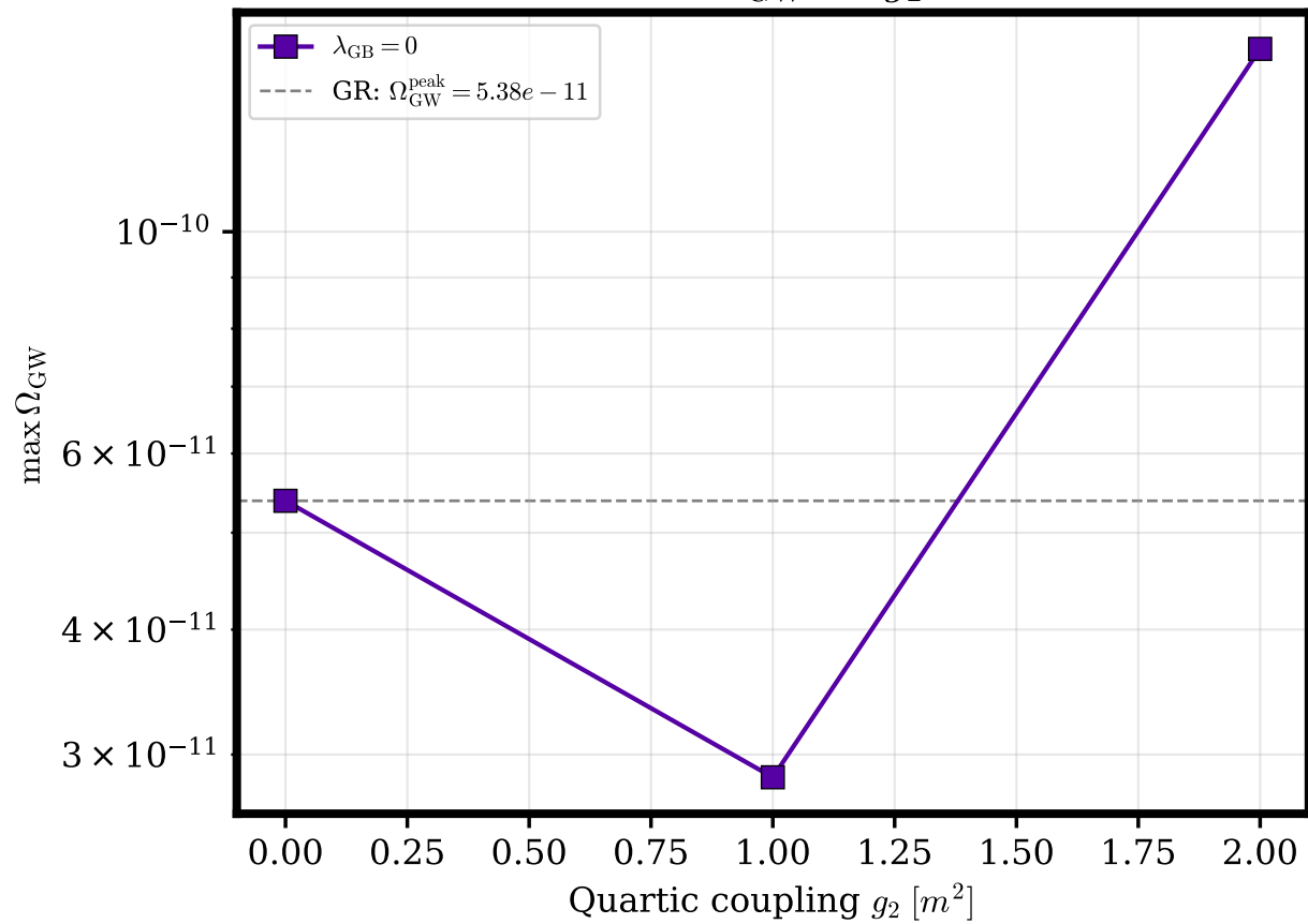
\max \Omega_{\text{GW}} vs g_2
