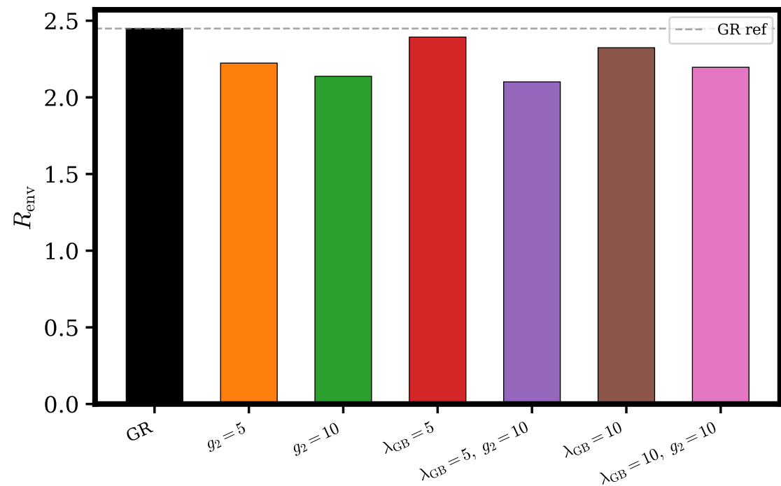
Oscillon parameters across couplings
