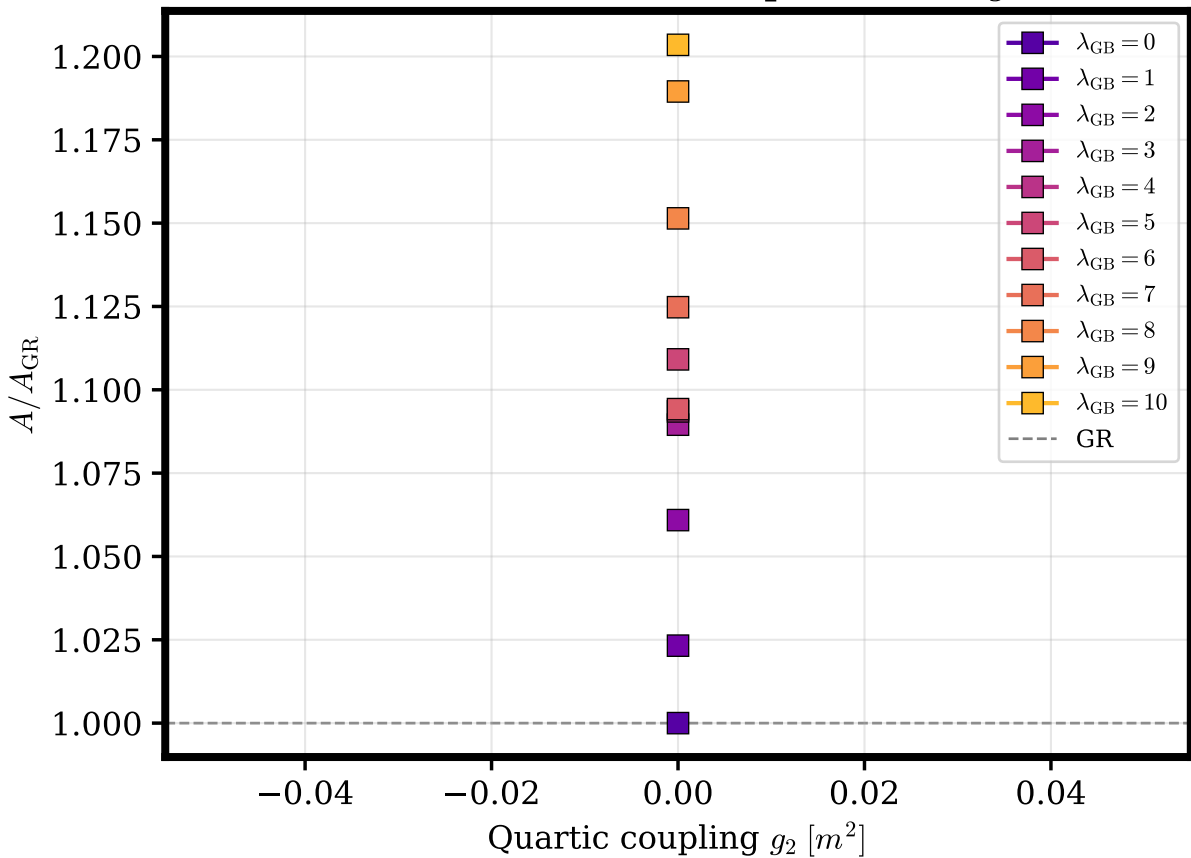
Relative oscillon amplitude vs g_2
