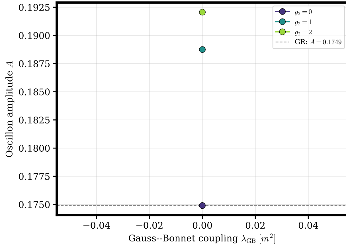
Oscillon amplitude vs \lambda_{\text{GB}}
