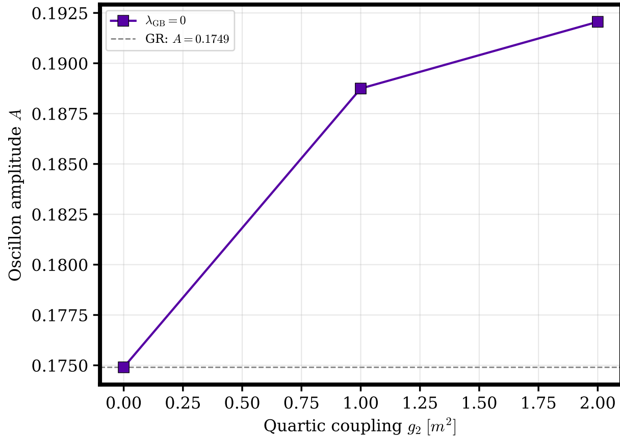
Oscillon amplitude vs g_2
