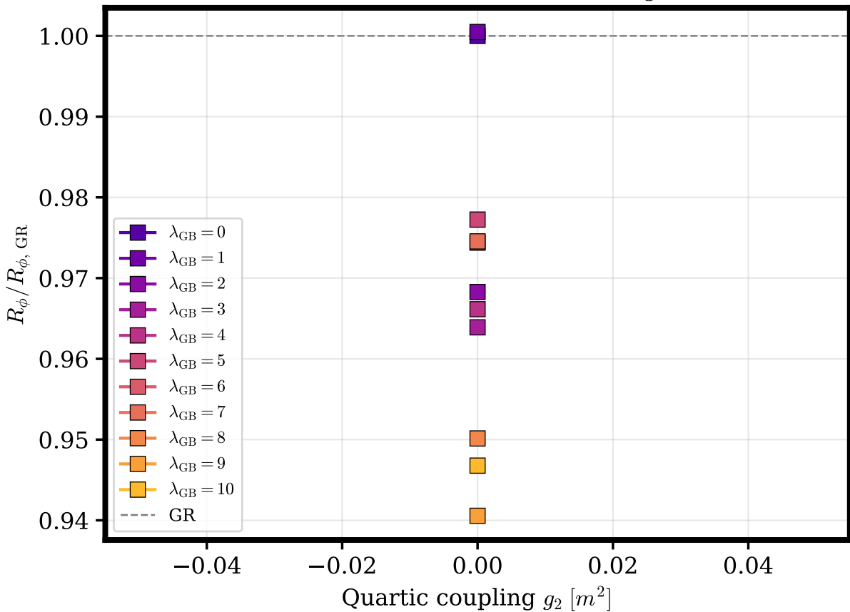
Relative field radius vs g_2
