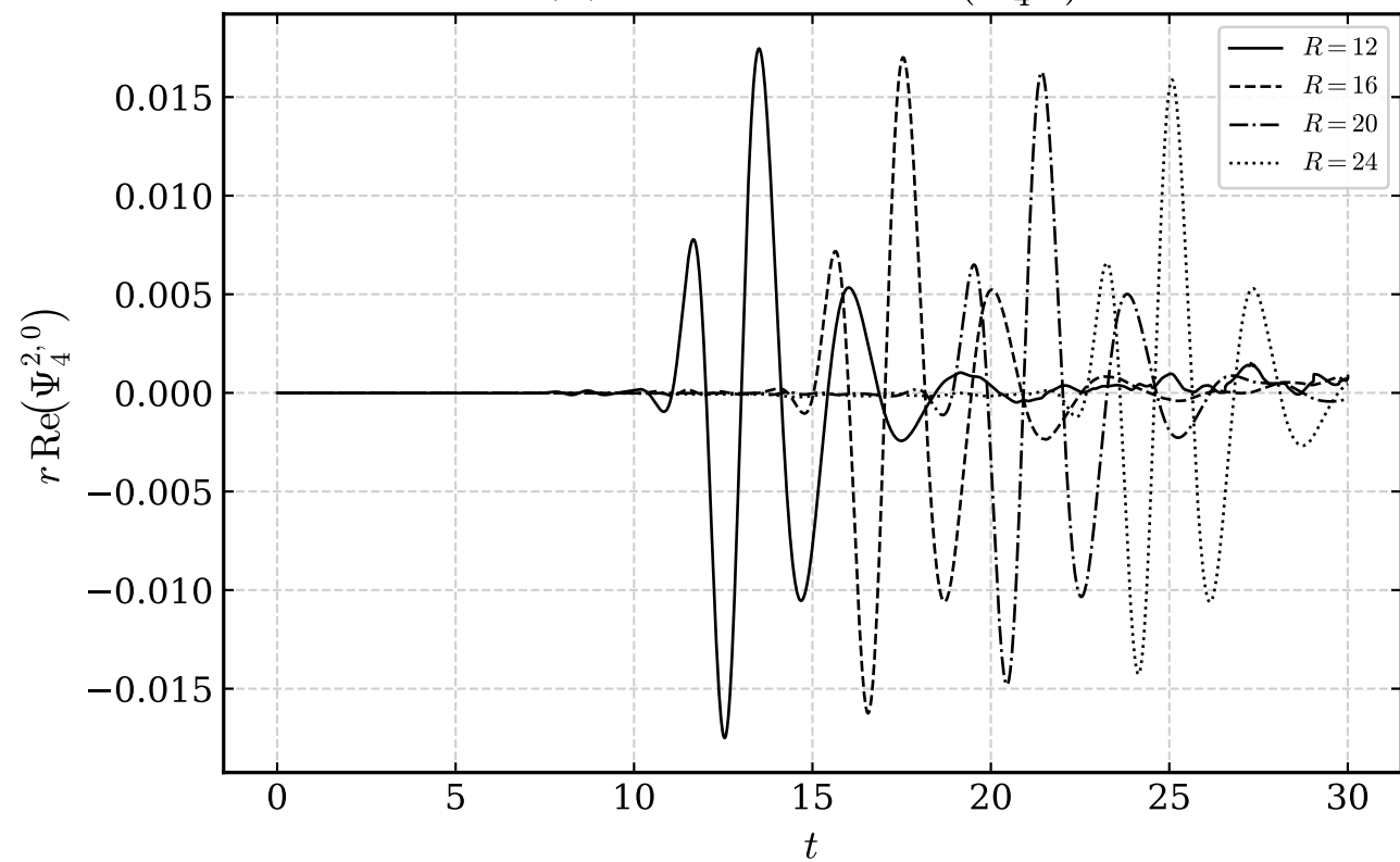
(a) Waveform r \text{Re}(\Psi_4^{2,0})
