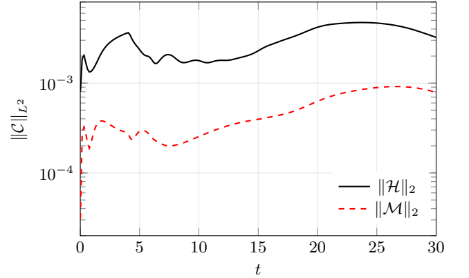
FIG. 9. Constraint norms in the headline RM run. The complete 3000-step diagnostic is plotted from a decimated table for typesetting only; maxima are evaluated from the full data.
