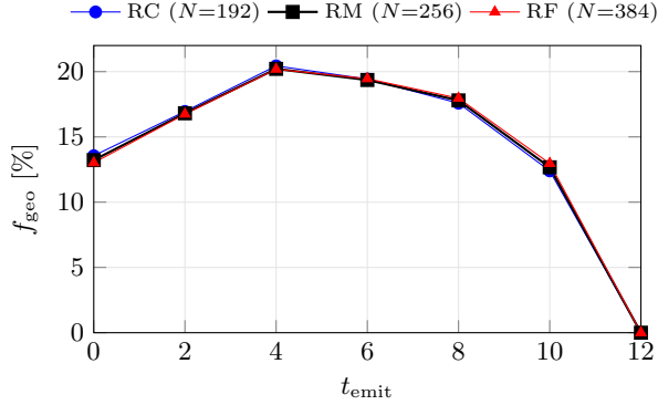
FIG. 8. Evolving null-geodesic emission sweeps ( t_{\text{emit}} = 0, 2, \dots, 12 ) for all three resolution-matrix runs; the metric evolves to t = 30 , but late launches lack enough remaining geometry for a complete transit. All runs peak at t_{\text{emit}} = 4 , just after PD pump-off, and agree within 0.26 percentage points. Every point shown has 5/5 rays reaching and passes the null-Hamiltonian quality gate.
