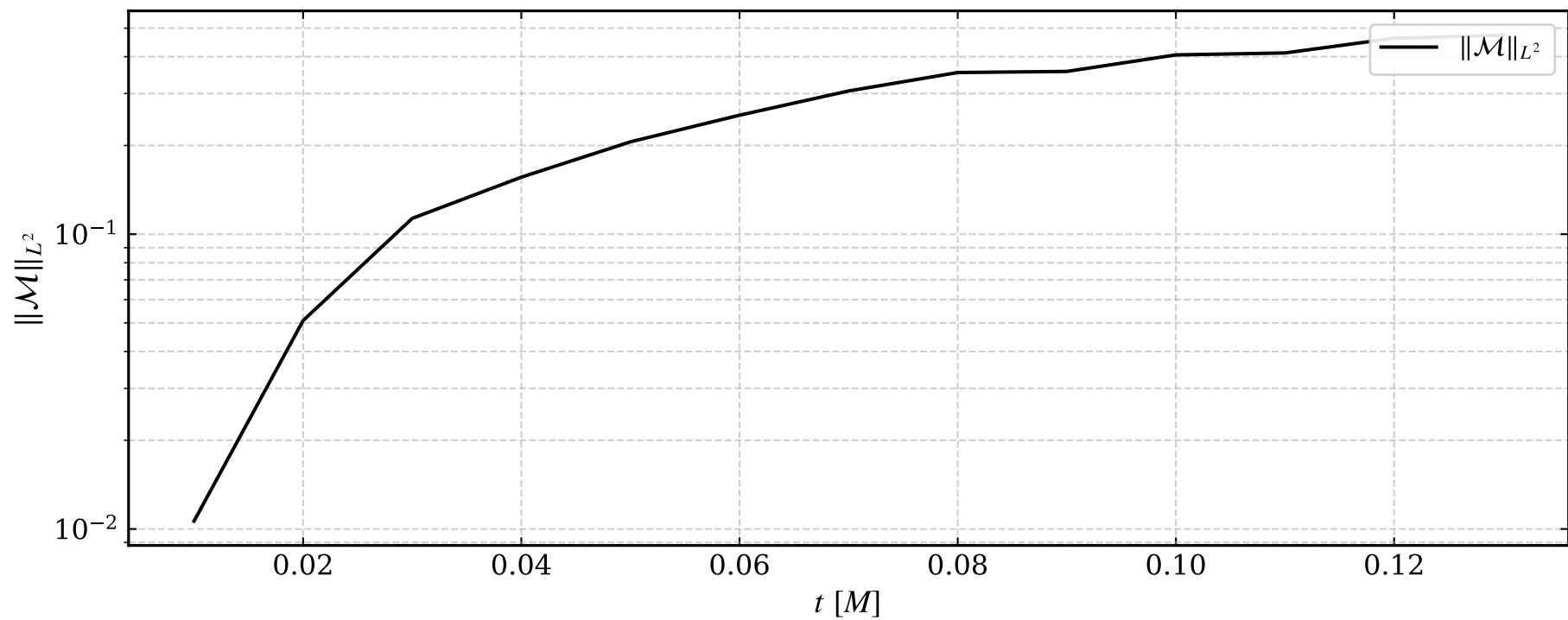
Momentum Constraint: \mathcal{M}^i
