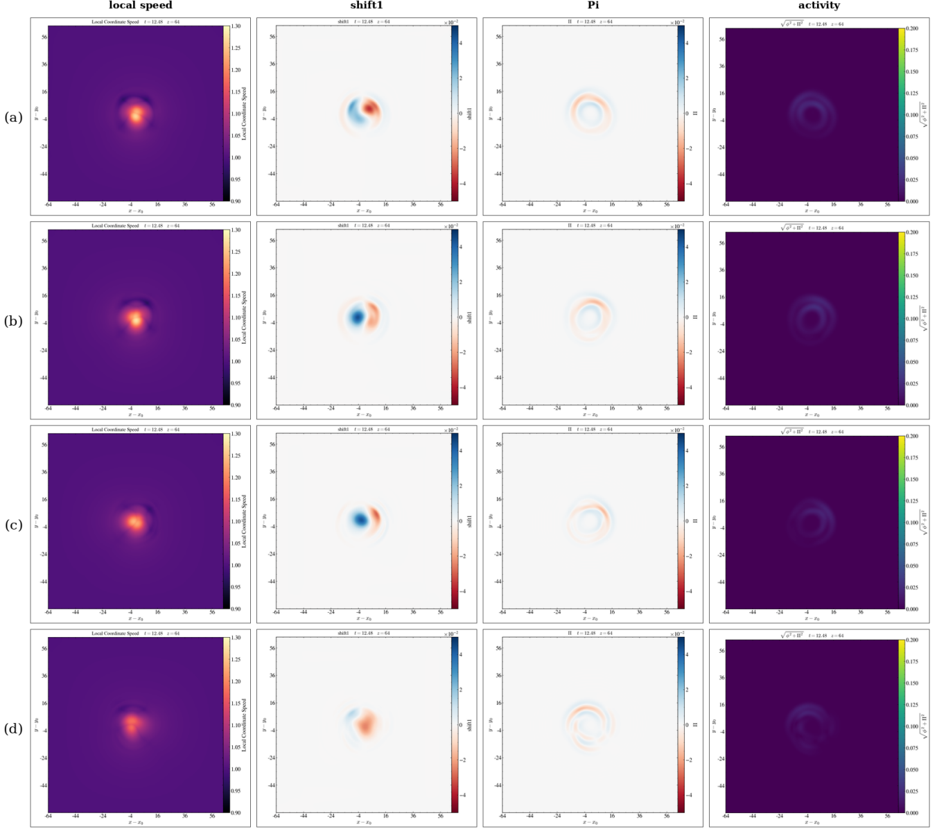
FIG. 5. High-resolution shell promotion, zoomed diagnostic slices ( L = 128 , N_{\text{full}} = 256 ). Rows show (a) eval_000106 , the final HQ winner; (b) eval_000117 , the strongest backup; (c) eval_000094 , the best channel/shift geometry; and (d) eval_000011 , the search-scale leader. Columns show local coordinate light speed, shift component \beta^x , scalar momentum \Pi , and scalar activity. These frames are taken from the visually diagnostic mid-run slice ( t \simeq 12.5 ) rather than the final score slice, where the scalar matter has largely dispersed; the final quantitative verdict is the t = 50.01 table. The channel-leaning candidates show stronger organized shift and matter-current structure than eval_000011 .
