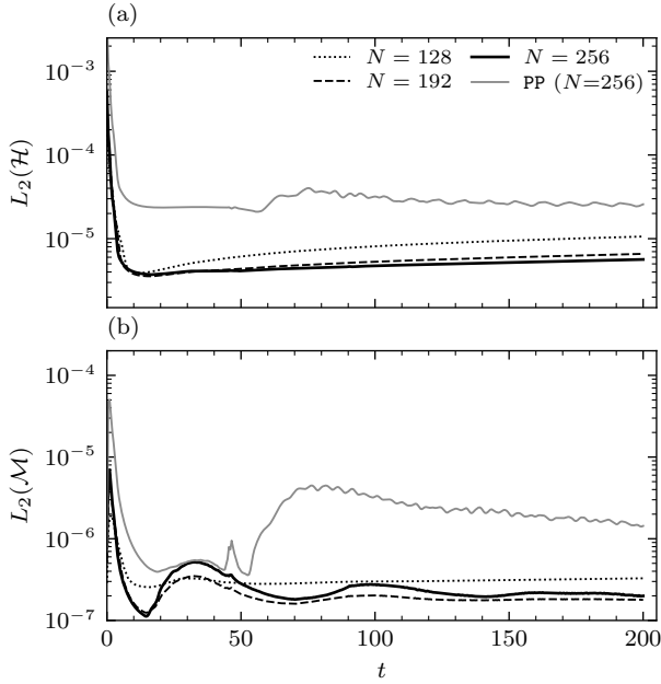
FIG. 10. Constraint norms for the headline cell’s resolution ladder (line styles as in Fig. 6) and the merging PP control at the finest grid (gray). (a) Hamiltonian, L_2 over the domain: finer grids start worse (initial-data interpolation noise) and evolve better. (b) Momentum, L_2 .
