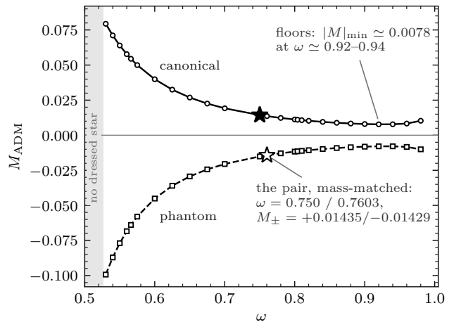
FIG. 2. ADM masses of the spherical stars against oscillation frequency at the working couplings. Lower \omega means deeper binding and larger |M_{\text{ADM}}| ; at equal frequency the phantom star is the heavier in magnitude, its repulsive self-gravity spreading it over more volume. Stars: the campaign pair—canonical at \omega = 0.750 , phantom returned to \omega = 0.7603 so the mass magnitudes match to 0.4%. Both branches have a floor : no star on either side is lighter than \simeq 0.54 of the campaign mass, and neither branch has a bound star at \omega = 1 —the bound that shapes the mass-scaling ladder of Sec. VF.
