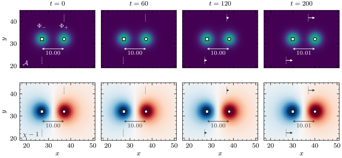
FIG. 3. The runaway in the headline cell (PM, d_0 = 10 , \Delta x = 0.25 ), z = 0 plane, at t = 0, 60, 120, 200 . Top: scalar-field activity \mathcal{A} = \sum_s (|\Phi_s|^2 + |\Pi_s|^2)^{1/2} , both sectors, projected. Bottom: \chi - 1 ; the phantom star is a hill ( \chi > 1 , left) and the canonical star a well ( \chi < 1 , right)—the model’s one sign, photographed. Open markers: the tracked cores (circle \Phi_+ , square \Phi_- ); dashed ticks mark the release positions x = 37 and 27 , arrows the displacement since release, and the bracketed number is the measured gap. Both stars move toward +x at constant acceleration while the gap holds to 1%.
