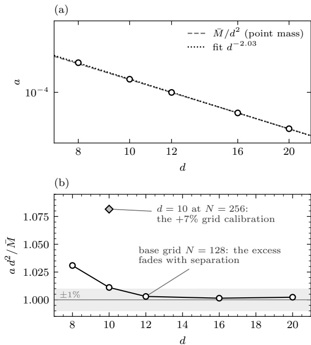
FIG. 5. The force law over d_0 = 8 –20 at the base grid. (a) Fitted acceleration against separation: the power-law fit gives d^{-2.03 \pm 0.01} ; the point-mass line \bar{M}/d^2 is indistinguishable at this scale. (b) a d^2 over the pair mass \bar{M} : the close-pair excess, +3.1% where the envelopes overlap most, decays monotonically and is gone by d = 16 —a finite-size correction behaving like one. The open diamond is the converged ( N = 256 ) value at d = 10 : refining the grid raises every acceleration by \sim 7\% (Sec. V C), a calibration common to the whole scan that cancels from the exponent and the trend.
