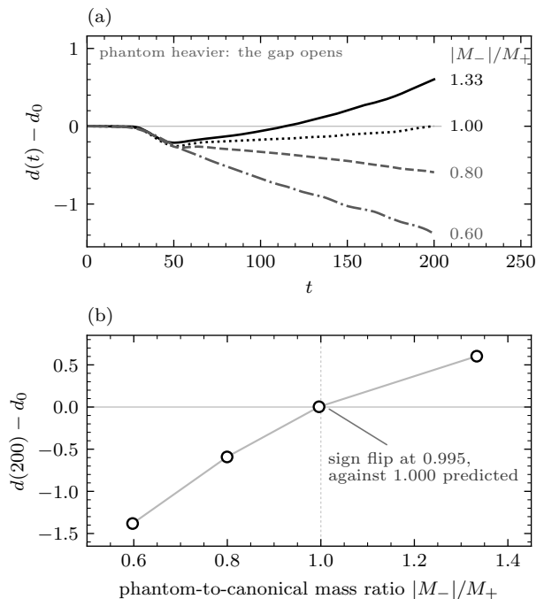
FIG. 8. The mass ladder: the matched pair and three retuned partners spanning a factor 2.2 in mass ratio. (a) Gap history: with a heavier phantom the gap opens , matched it holds, with a lighter phantom it closes , monotonically in the ratio. Every cell shares the same t \approx 50 gauge dip, so the gap is read late. (b) Gap change at t = 200 against the mass ratio, monotone through the four cells: the sign flip falls at ratio 0.995, against 1.000 predicted—the test no artefact survives, because an artefact can close a gap but cannot make the closing reverse according to which of two stars is heavier.
