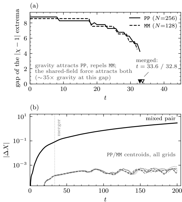
FIG. 7. The same-sign controls. (a) Gap between the two |\chi - 1| extrema—wells for PP, hills for MM—tracked frame by frame: both pairs fall together and merge, at t = 33.6 and 32.8 . Newtonian gravity’s sign is opposite between these two cells, so the force that sets their common clock is blind to the sign of the mass: the shared field’s overlap attraction, \sim 35\times gravity at this gap. The mixed pair has no shared field—gravity is its only channel. (b) Through plunge, merger and ringdown, the PP/MM pair centroids (all grids) stay below 8 \times 10^{-4} —four orders under the mixed pair’s drift. A configuration that cannot manufacture momentum even while merging is a stronger null than one that sits still.
