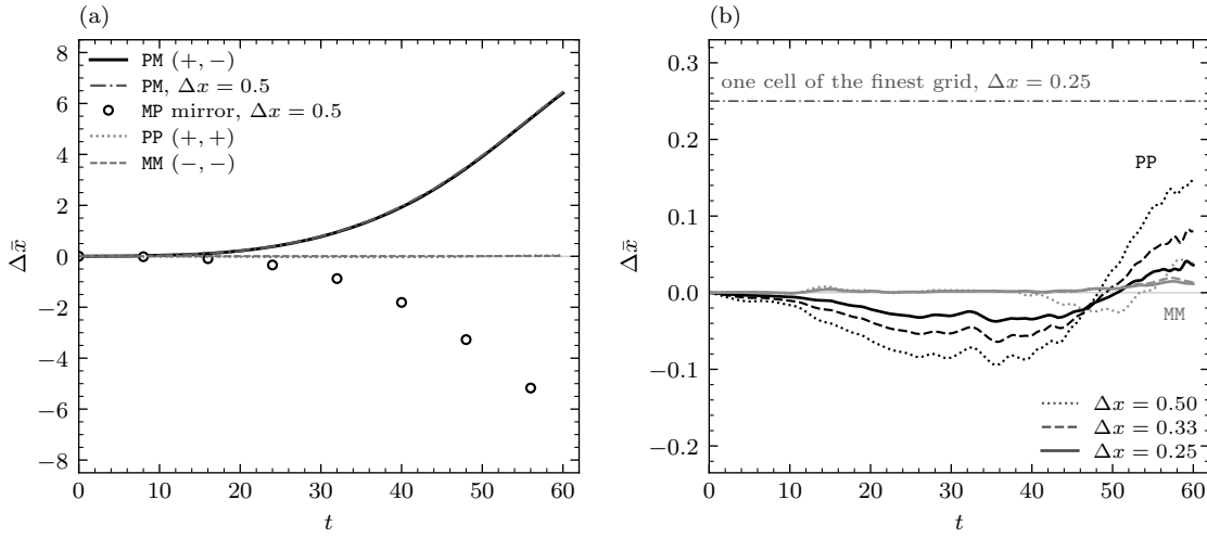
FIG. 5. The four sign assignments under identical numerics. (a) Pair-barycentre drift at d_0 = 8 : the mixed pair PM runs away to +6.41 at \Delta x = 0.25 and +6.45 at \Delta x = 0.5 , its space-reflected twin MP to -6.15 at the same \Delta x = 0.5 (a 4.7% asymmetry), while PP and MM stay on the axis. (b) The same-sign residuals magnified, at all three resolutions: PP reaches +0.036 and MM +0.012 at t = 60 —179 and 545 times smaller than the mixed pair, both below one cell width of the finest grid, and both shrinking as the grid is refined.
