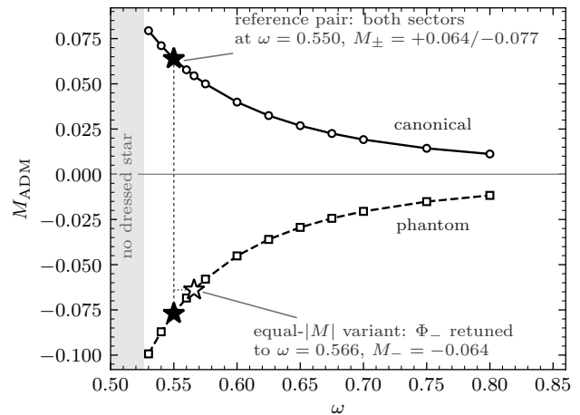
FIG. 2. ADM masses of the spherical stars against oscillation frequency, from Eqs. (6) at the working couplings: the canonical branch ( M_{\text{ADM}} > 0 ) and the phantom branch ( M_{\text{ADM}} < 0 ). Lower \omega means deeper binding and larger |M_{\text{ADM}}| ; in the shaded region the solver finds no dressed star. At equal frequency the phantom star is the heavier in magnitude (20.3% at \omega = 0.550 , 4.3% at \omega = 0.80 ), its repulsive self-gravity spreading it over more volume. Filled stars: the reference pair, both sectors at \omega = 0.550 . Open star: the equal- |M_{\text{ADM}}| variant, whose phantom is retuned to \omega = 0.56598 so that M_- = -0.063950 matches the canonical star to one part in 10^5 .
