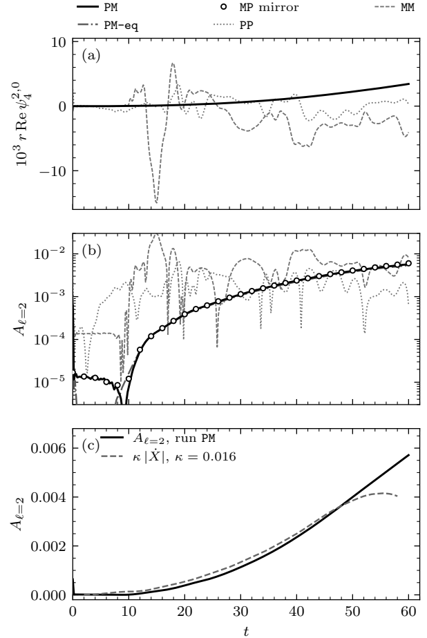
FIG. 7. The \ell = 2 Weyl signal at R = 16 , campaign cells at \Delta x = 0.25 (the mirror overlay exists only at \Delta x = 0.5 ). (a) The raw waveform r \text{Re} \psi_4^{2,0} : in the mixed run a monotone, chirpless ramp; in the same-sign controls a non-secular wander. (b) Total amplitude A_{\ell=2}(t) : the mixed pairs climb by two orders of magnitude ( 232\times for PM, 350\times for the equal- |M| rerun, 481\times for the mirror, 122\times in the reference d_0 = 12 cell) while the controls do not. (c) The amplitude against the rescaled pair speed \kappa|\dot{X}| : correlation 0.996 over 5 \leq t \leq 55 with \kappa \approx 0.016 —the near-zone quadrupole rises in lockstep with the runaway, not with the field frequency.
