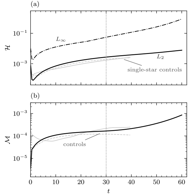
FIG. 8. Constraint monitoring: reference run PM (black) against the single-star controls (light gray; solid canonical, dashed phantom). (a) Hamiltonian constraint \mathcal{H} : composite L_2 norms (solid) and the reference run’s L_\infty (dash-dotted). (b) Momentum constraint \mathcal{M} , L_2 . The equal- |M| rerun lies indistinguishably under the black curves and is omitted; the dotted line marks the clean-window edge t = 30 .
