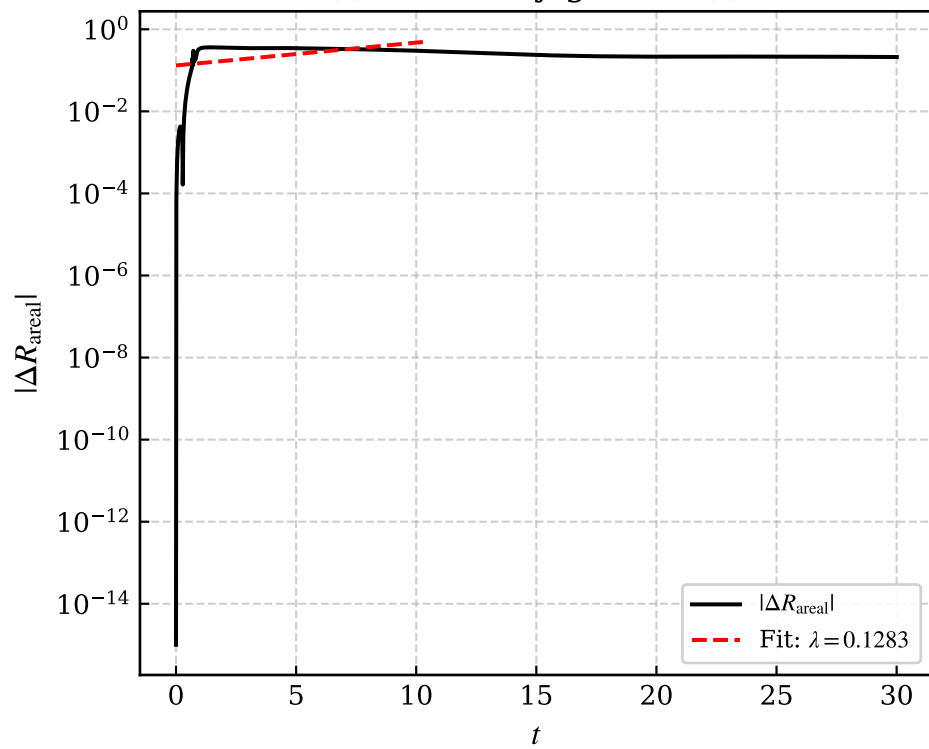
(l) Instability growth ( \lambda )
