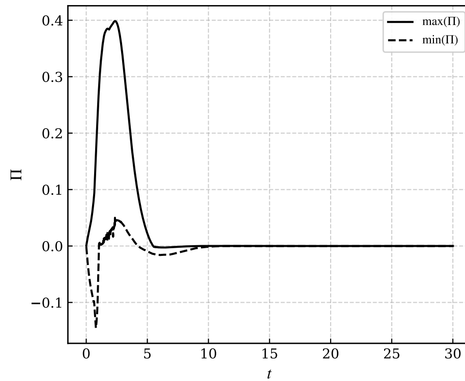
(k) Scalar field momentum \Pi
