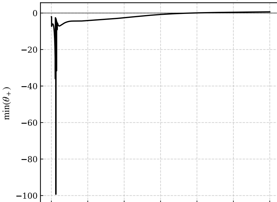
(h) Expansion velocity
