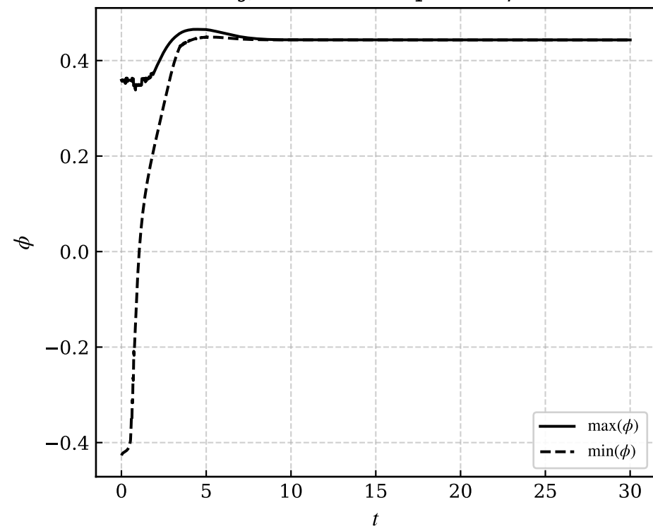
(j) Scalar field profile \phi
