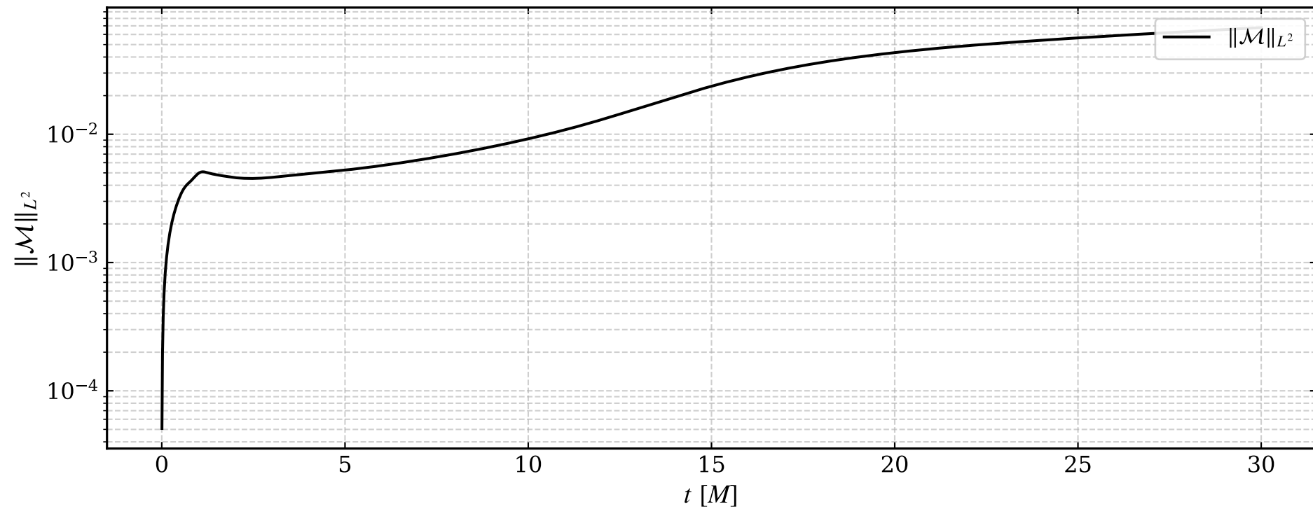
Momentum Constraint: \mathcal{M}^i
