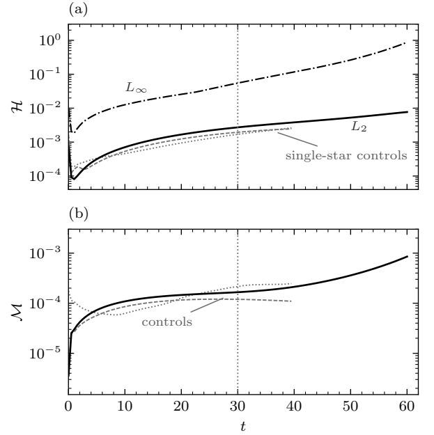
FIG. 9. Constraint monitoring: reference run PM (black) against the single-star controls (gray; dotted canonical, tightly dashed phantom). (a) Hamiltonian constraint \mathcal{H} : composite L_2 norms (solid) and the reference run’s L_\infty (dash-dotted). (b) Momentum constraint \mathcal{M} , L_2 . The equal- |M| rerun lies indistinguishably under the black curves and is omitted; the dotted line marks the clean-window edge t = 30 .
