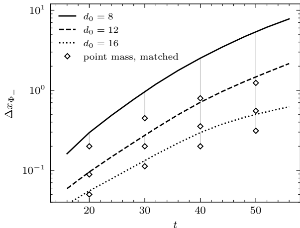
FIG. 7. Separation scaling of the phantom drift (the trustworthy sector; Sec. VII). Curves: NR runs at d_0 = 8, 12, 16 ; diamonds: each run’s own matched point-mass integration, tied to its curve at equal times (Table IV).
