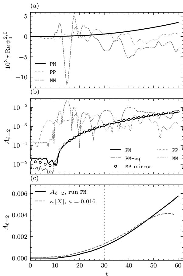
FIG. 8. The \ell = 2 Weyl signal. (a) The raw waveform r \text{Re} \psi_4^{2,0} on the R = 16 shell: in the mixed run a monotone, chirpless ramp; in the same-sign controls (dotted PP, dashed MM) an oscillatory wander with no secular trend. (b) Total spin-weighted amplitude A_{\ell=2}(t) on the same shell: the mixed pairs (reference PM solid, equal- |M| rerun dash-dotted, mirrored run MP circles) climb smoothly to 300–800 times their early-time floors. (c) The reference-run amplitude against the pair speed |\dot{X}| (barycentre-midpoint drift rate, rescaled by the fitted \kappa ): correlation 0.995 over 5 \leq t \leq 55 . Beyond the clean-window edge (dotted line) the measured speed is biased low by the halo (Sec. VII) while the curvature amplitude keeps rising.
