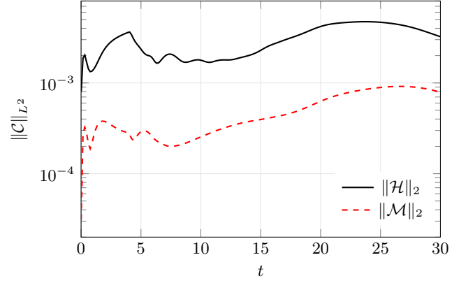
FIG. 13. Constraint norms in the headline RM run. The complete 3000-step diagnostic is plotted from a decimated table for typesetting only; maxima are evaluated from the full data.
