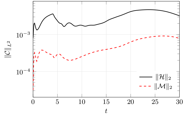
FIG. 10. Constraint norms in the headline RM run. The complete 3000-step diagnostic is plotted from a decimated table for typesetting only; maxima are evaluated from the full data.
