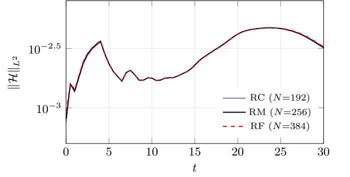
FIG. 9. Hamiltonian constraint norm across the Richardson ladder. The three resolutions overlie closely; the observed order extracted from Eq. (11) in the ignition window is p_{\mathcal{H}} \approx 3.3 (median).
