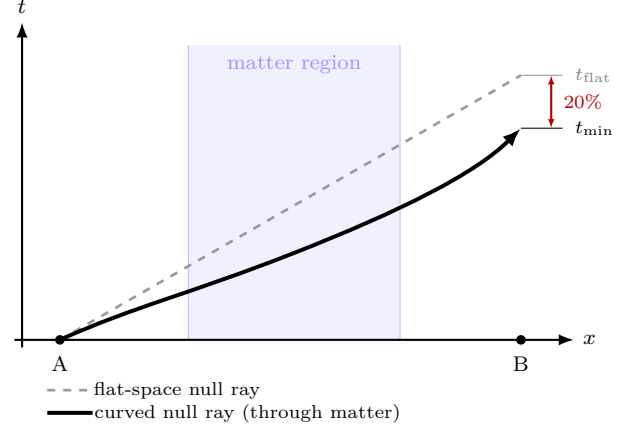
FIG. 11. Spacetime diagram of the null-geodesic shortcut. A photon emitted at A propagates toward receiver B. In flat space (dashed) the transit takes t_{\text{flat}} . Inside the Q-ball matter region (shaded band) the geometry bends null paths so that the ray through the curved spacetime (solid) arrives at B in t_{\text{min}} < t_{\text{flat}} . The bracket on the right marks the \sim 20\% coordinate-time saving. The ray never leaves its local light cone.
