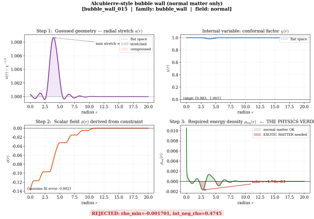
FIG. 5. Rejected normal-matter bubble-wall candidate. The radial bubble-wall shape is small and smooth, but the required energy density still dips below zero. This illustrates why a visually mild deformation of \chi(r) can still be physically exotic.
