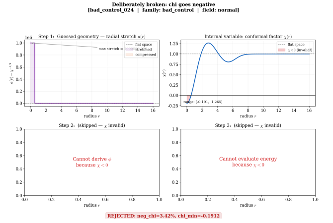
FIG. 6. Rejected bad-control candidate. The conformal factor \chi(r) becomes negative, so the spatial metric \gamma_{ij} = \chi^{-1}\delta_{ij} is invalid before any matter reconstruction or evolution.
