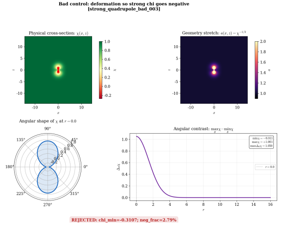
FIG. 9. Rejected non-spherical bad control. The same type of angular deformation is made too strong. The cross-section shows regions where \chi < 0 , which makes \gamma_{ij} = \chi^{-1}\delta_{ij} invalid. This is rejected before any constraint solve or C++ evolution because the metric itself is not admissible.
