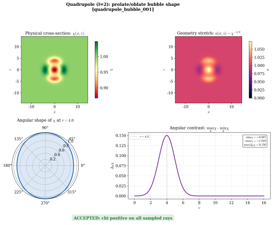
FIG. 8. Accepted non-spherical quadrupole candidate. The l = 2 mode creates a prolate/oblate deformation: the shape is different along the poles than around the equator. The polar panel makes the broken spherical symmetry visible, while the contrast panel shows that the deformation is localized near one radial shell.
