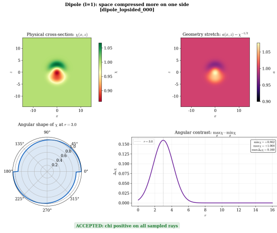
FIG. 7. Accepted non-spherical dipole candidate. The l = 1 mode makes the geometry lopsided: one side of the cross-section is compressed/stretched differently from the other. The key result is that \chi stays positive everywhere in the sampled section, so the metric is geometrically valid at this first ray-check level.
