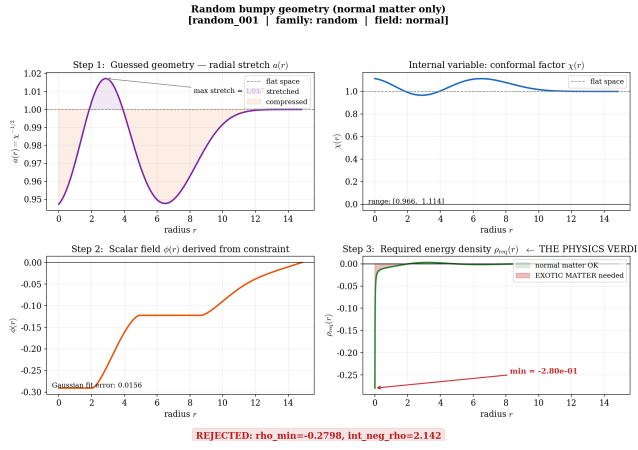
FIG. 4. Rejected normal-matter random candidate. The guessed geometry and derived scalar field are well-defined, but \rho_{\text{req}}(r) becomes negative. Since this candidate is in the normal-matter class, it is rejected as rejected_exotic_energy .
