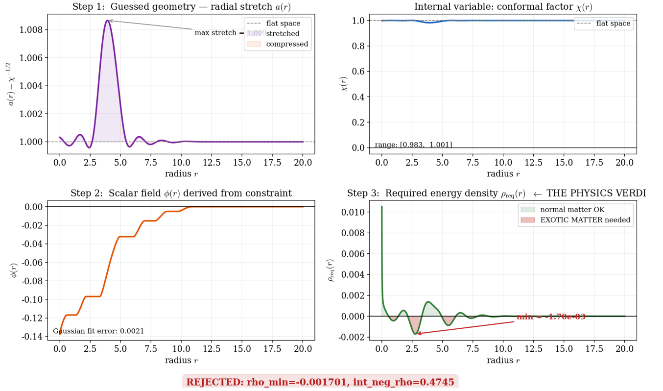
FIG. 5. Rejected normal-matter bubble-wall candidate. The radial bubble-wall shape is small and smooth, but the required energy density still dips below zero. This illustrates why a visually mild deformation of \chi(r) can still be physically exotic.
