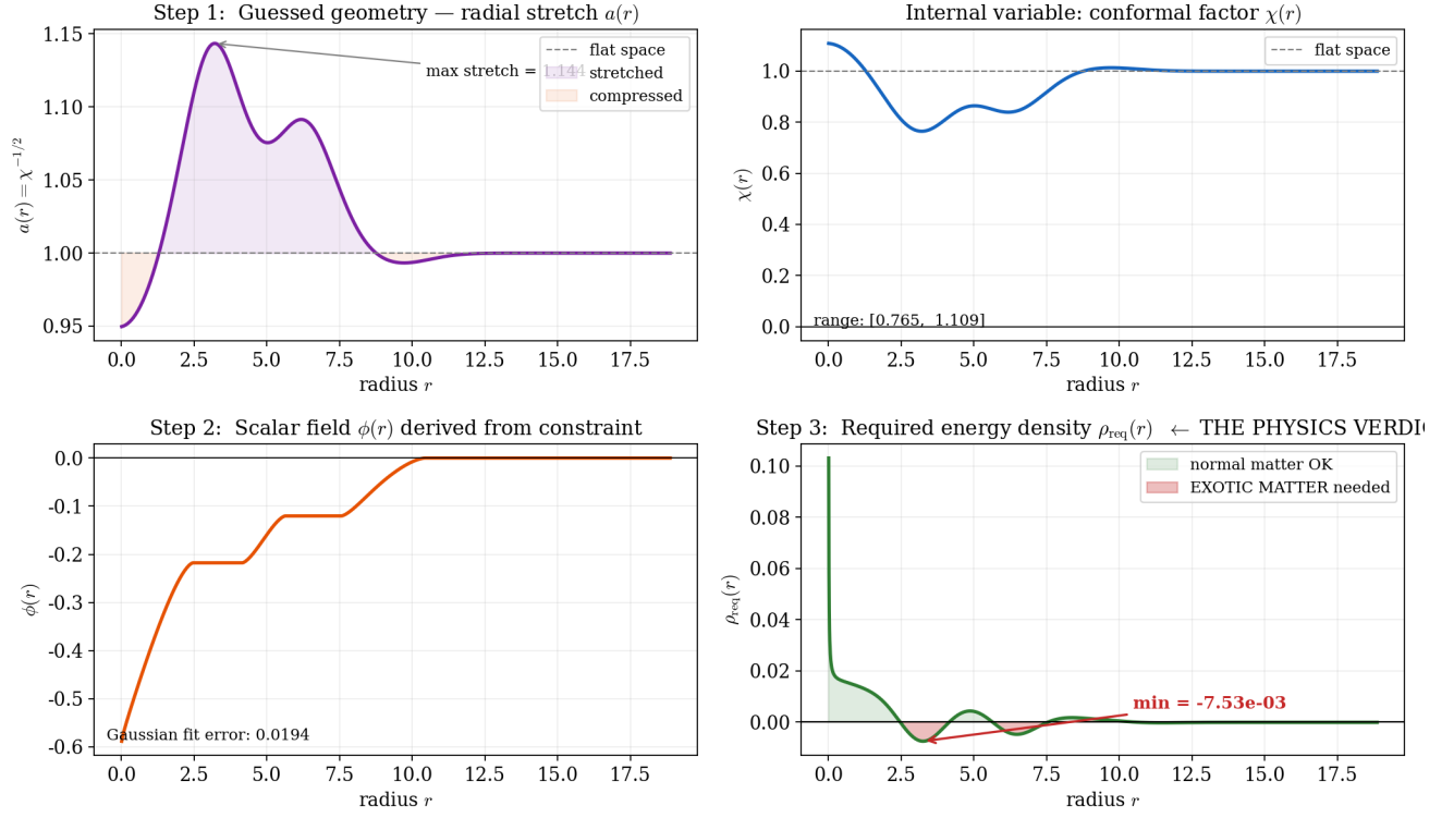
FIG. 2. Accepted phantom random candidate. The geometry is numerically constructible and the pre-flight constraints remain controlled. The required energy density contains negative regions, so it is accepted only in the phantom/exotic-matter class.
