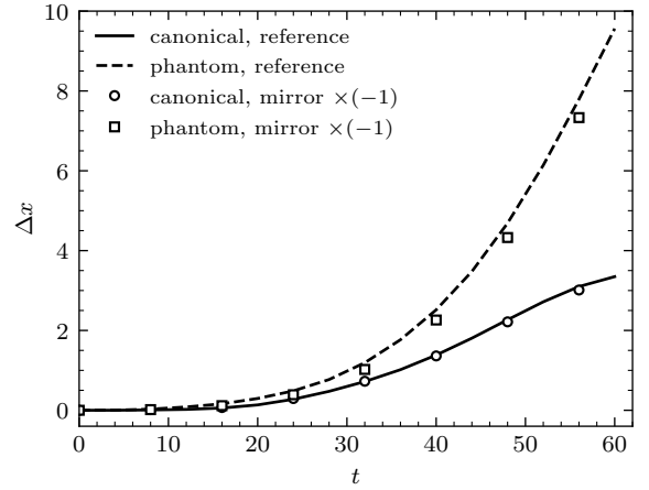
FIG. 6. Mirror control. Lines: reference run PM (canonical solid, phantom dashed); open markers: the mirrored run MP’s drift multiplied by -1 (circles canonical, squares phantom). Reflecting the configuration reflects the trajectory to a few percent.
