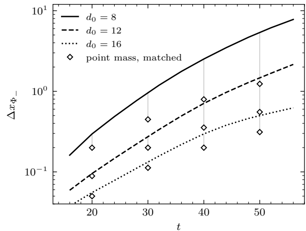
FIG. 7. Separation scaling of the phantom drift (the trustworthy sector; Sec. VI). Curves: NR runs at d_0 = 8, 12, 16 ; diamonds: each run’s own matched point-mass integration, tied to its curve at equal times (Table IV).
