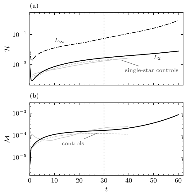
FIG. 8. Constraint monitoring: reference run PM (black) against the single-star controls (light gray; solid canonical, dashed phantom). (a) Hamiltonian constraint \mathcal{H} : composite L_2 norms (solid) and the reference run’s L_\infty (dash-dotted). (b) Momentum constraint \mathcal{M} , L_2 . The equal- |M| rerun lies indistinguishably under the black curves and is omitted; the dotted line marks the clean-window edge t = 30 .
