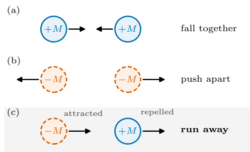
FIG. 1. Bondi’s sign rules for two bodies released at rest, in the style of Forward’s analysis [5]. Every body here has positive inertial and passive mass; only the active (source) mass carries a sign—negative for the dashed bodies. (a) Two positive-mass stars attract each other and fall together; (b) two negative-mass stars repel each other and push apart. In both cases the forces oppose, and the pair’s centre stays put. (c) The mixed pair—the Bondi dipole: the positive star is repelled by the negative one, the negative star is attracted by the positive one, so both forces point the same way and the pair runs off together, carrying zero total momentum in the signed bookkeeping. Each row is realized as a run of the matrix in Table I.
