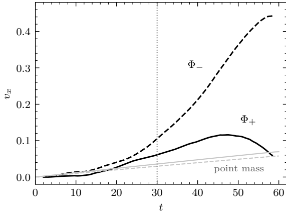
FIG. 5. Barycentre velocities in run PM, in code units ( c = 1 ): centred differences of the continuously sampled barycentre stream over \pm 2 time units (canonical solid, phantom dashed; light gray: the matched point-mass model). The dotted line marks the clean-window edge t = 30 ; beyond it the halo bias (Sec. VI) depresses the canonical curve.
