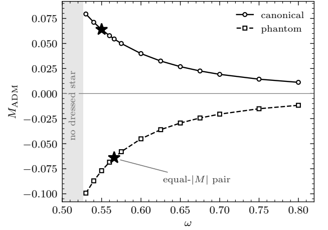
FIG. 2. ADM masses of the spherical stars against the field oscillation frequency \omega , from Eqs. (5) at the working couplings: canonical stars ( M_{\text{ADM}} > 0 , circles) and phantom stars ( M_{\text{ADM}} < 0 , squares). Lower frequency means deeper binding and larger |M_{\text{ADM}}| ; in the shaded region the solver finds no gravitationally dressed star. At equal frequency the phantom star is the heavier in magnitude (20% at \omega = 0.55 , 4% at \omega = 0.80 ), its repulsive self-gravity spreading it over more volume. Stars ( \star ): the equal- |M_{\text{ADM}}| pair of run PM-eq, matched to one part in 10^5 .
