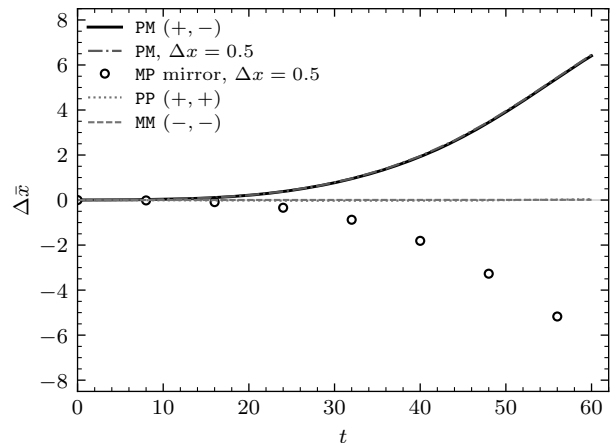
FIG. 5. The four sign assignments under identical numerics: pair-barycentre drift at d_0 = 8 . The mixed pair PM runs away to +6.41 at \Delta x = 0.25 and +6.45 at \Delta x = 0.5 , its space-reflected twin MP to -6.15 at the same \Delta x = 0.5 (a 4.7% asymmetry), while PP and MM stay on the axis at +0.036 and +0.012 —below one cell width of the finest grid, and shrinking under refinement (Fig. 6b).
