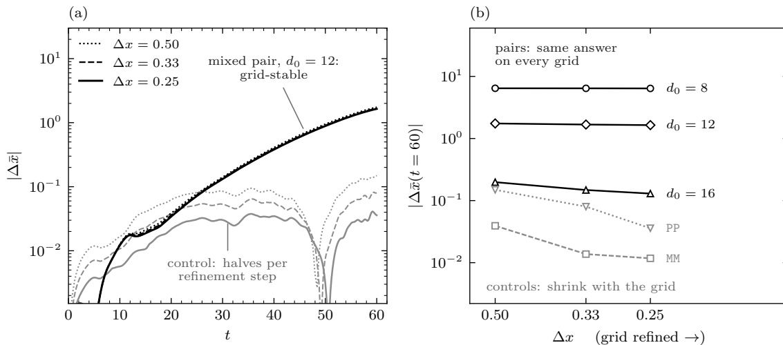
FIG. 6. The convergence study. (a) The reference cell’s resolution ladder in time (dotted \Delta x = 0.50 , dashed 0.33, solid 0.25) against the PP control’s ladder: the mixed-pair curves lie on top of one another while the control’s residual drift roughly halves at every refinement step. (b) The same data as a refinement sequence— |\Delta\bar{x}| at t = 60 against grid spacing, grid refined to the right—for every family. The mixed pairs sit on plateaus (spread 0.5% at d_0 = 8 , 6.3% at d_0 = 12 ) while the same-sign controls fall towards zero. The under-resolved d_0 = 16 family is the exception that shows the test works: its 53% spread is why it is quoted as a bound.
