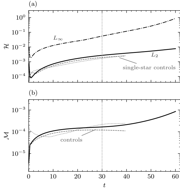
FIG. 8. Constraint monitoring: reference run PM (black) against the single-star controls (gray; dotted canonical, tightly dashed phantom). (a) Hamiltonian constraint \mathcal{H} : composite L_2 norms (solid) and the reference run’s L_\infty (dash-dotted). (b) Momentum constraint \mathcal{M} , L_2 . The equal- |M| rerun lies indistinguishably under the black curves and is omitted; the dotted line marks the clean-window edge t = 30 .
