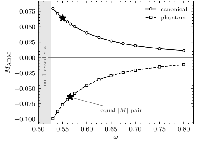
FIG. 2. ADM masses of the spherical stars against the field oscillation frequency \omega , from Eqs. (6) at the working couplings: canonical stars ( M_{\text{ADM}} > 0 , circles) and phantom stars ( M_{\text{ADM}} < 0 , squares). Lower frequency means deeper binding and larger |M_{\text{ADM}}| ; in the shaded region the solver finds no gravitationally dressed star. At equal frequency the phantom star is the heavier in magnitude (20% at \omega = 0.55 , 4% at \omega = 0.80 ), its repulsive self-gravity spreading it over more volume. Stars ( \star ): the equal- |M_{\text{ADM}}| pair of run PM-eq, matched to one part in 10^5 .
