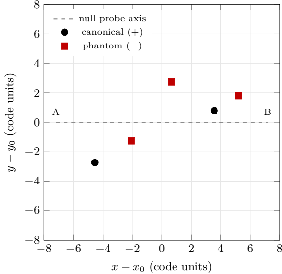
FIG. 9. Top-down ( x - y ) projection of the candidate-146 initial lump centers at true grid scale (box center (x_0, y_0) = (64, 64) ; no magnification). Black circles are the two canonical (+) lumps, red squares the three phantom (-) lumps [signs (+, -, -, +, -)]. The dashed line is the x -directed null-probe corridor from emitter A to receiver B ( |x - x_0| \leq 7.2 ). Compared with Fig. 8, this panel shows the actual spatial extent of the shell: the five solitons occupy a region a few code units across, comparable to the corridor half-length.
