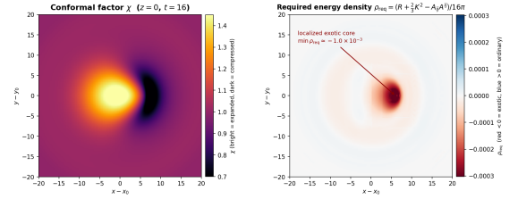
FIG. 2. The warp dipole is held by a localized exotic core, with negligible ordinary matter. Left: conformal factor \chi at z = 0 , t = 16 (bright = expanded, dark = compressed). Right: the geometric required energy density \rho_{\text{req}} of Eq. (32) on the same slice (red < 0 exotic, blue > 0 ordinary, shared symmetric scale). The energy-condition violation needed to sustain the geometry is concentrated in one compact core ( \min \rho_{\text{req}} \approx -1.0 \times 10^{-3} ) coincident with the compression crescent; the surrounding domain is near-vacuum and the faint outer ring is the weak outgoing K -wave (junk radiation), not localized matter.
