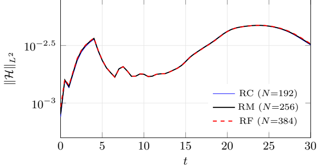
FIG. 9. Hamiltonian constraint norm across the Richardson ladder. The three resolutions overlie closely; the observed order extracted from Eq. (11) in the ignition window is p_{\mathcal{H}} \approx 3.3 (median).
