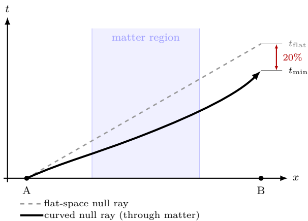
FIG. 11. Spacetime diagram of the null-geodesic shortcut. A photon emitted at A propagates toward receiver B. In flat space (dashed) the transit takes t_{\text{flat}} . Inside the Q-ball matter region (shaded band) the geometry bends null paths so that the ray through the curved spacetime (solid) arrives at B in t_{\text{min}} < t_{\text{flat}} . The bracket on the right marks the \sim 20\% coordinate-time saving. The ray never leaves its local light cone.
