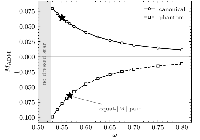
FIG. 1. ADM masses of the spherical stars against the field oscillation frequency \omega , from Eqs. (5) at the working couplings: canonical stars ( M_{\text{ADM}} > 0 , circles) and phantom stars ( M_{\text{ADM}} < 0 , squares). Lower frequency means deeper binding and larger |M_{\text{ADM}}| ; in the shaded region the solver finds no gravitationally dressed star. At equal frequency the phantom star is the heavier in magnitude (20% at \omega = 0.55 , 4% at \omega = 0.80 ), its repulsive self-gravity spreading it over more volume. Stars (*): the equal- |M| pair of run PM-eq, matched to one part in 10^5 .
