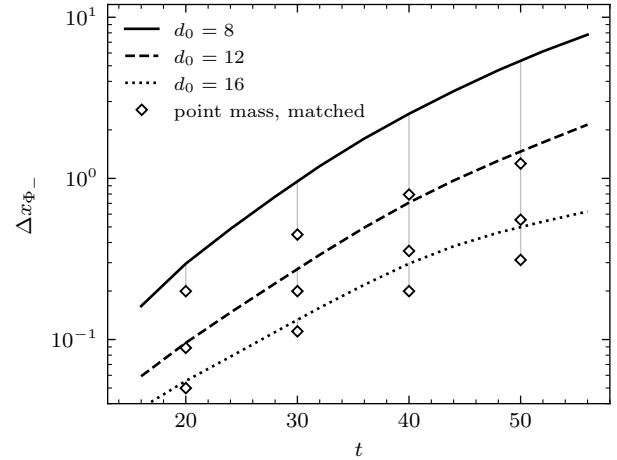
FIG. 6. Separation scaling of the phantom drift (the trustworthy sector; Sec. VI). Curves: NR runs at d_0 = 8, 12, 16 ; diamonds: each run's own matched point-mass integration, tied to its curve at equal times (Table IV).
