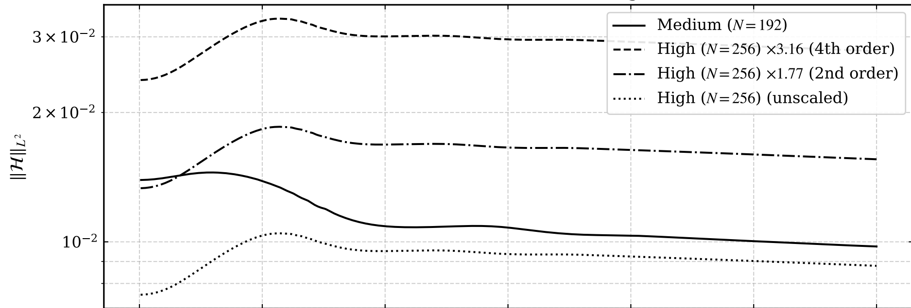
Momentum Constraint Convergence: \mathcal{M}^i
