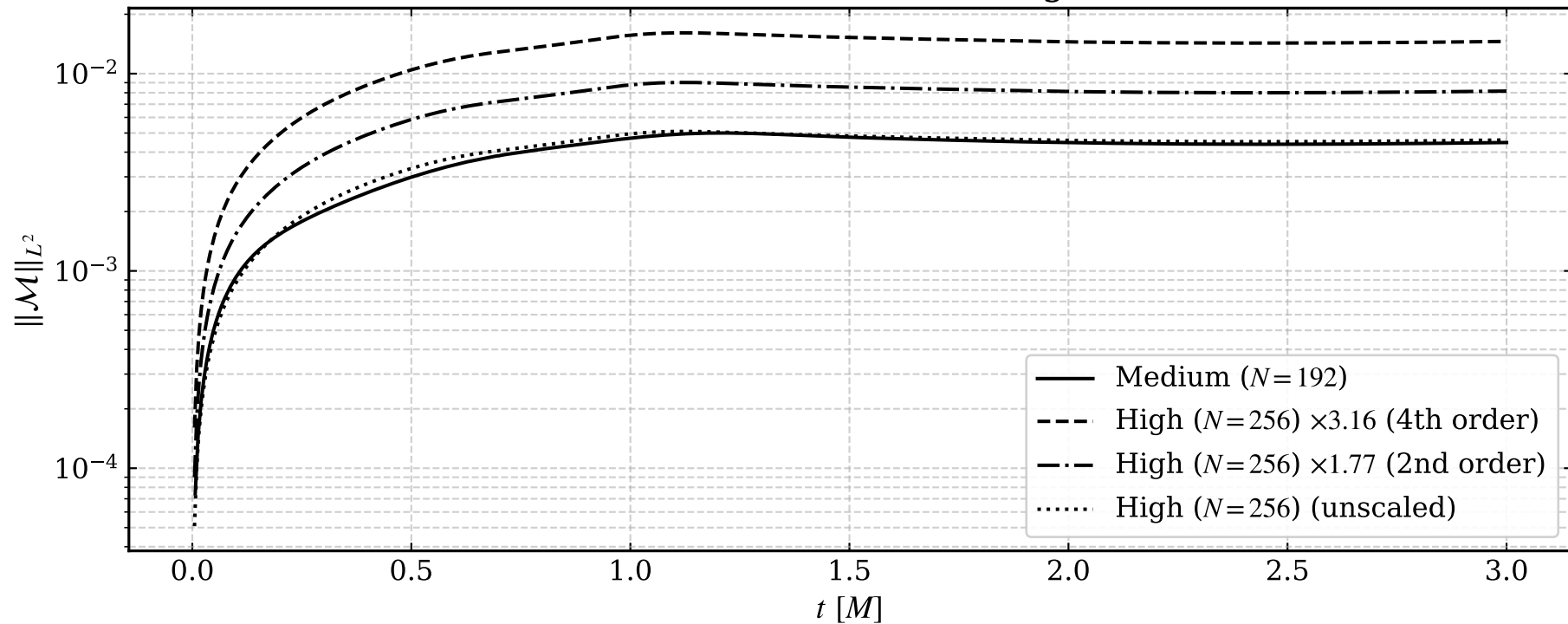
Momentum Constraint Convergence: \mathcal{M}^i
