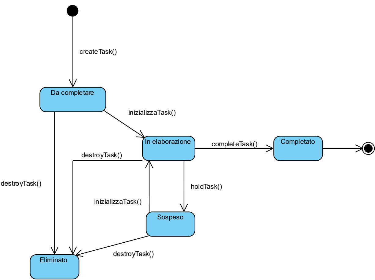
Statechart diagram
