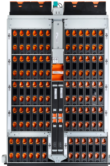
Ultrastar Data60 Hybrid Storage Platform
