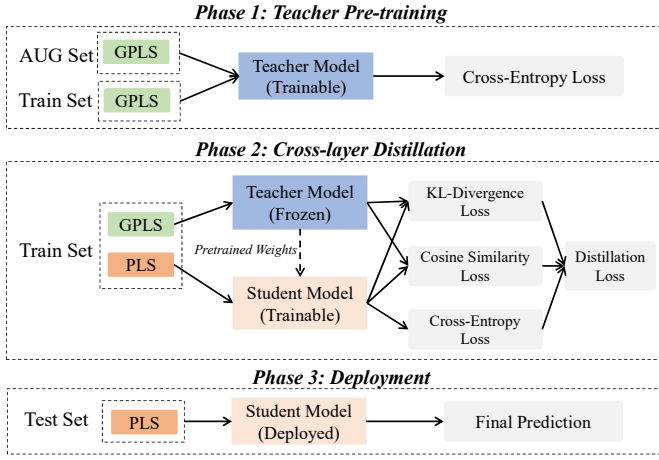
Fig. 6. Cross-layer feature alignment architecture.
