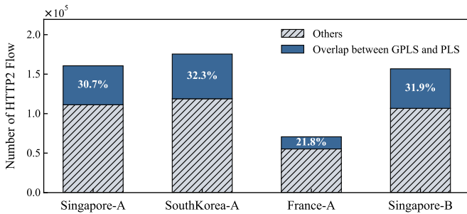
Fig. 10. Overlap between GPLS and real PLS across datasets.
