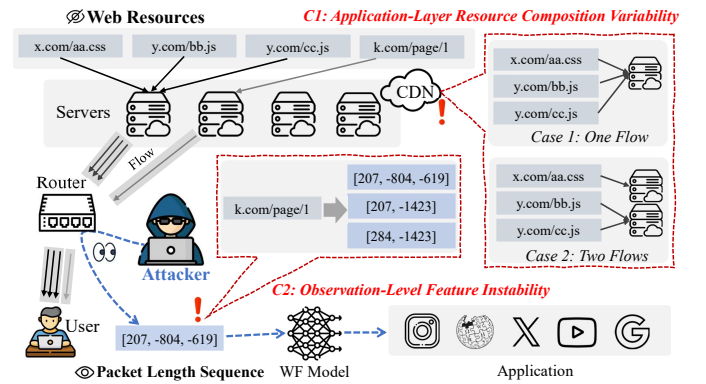
Fig. 1. Overview of a WF attack scenario and its two major generalization challenges. Blue dashed lines denote the attacker's workflow, and red dashed regions indicate the challenges faced by the attacker.
