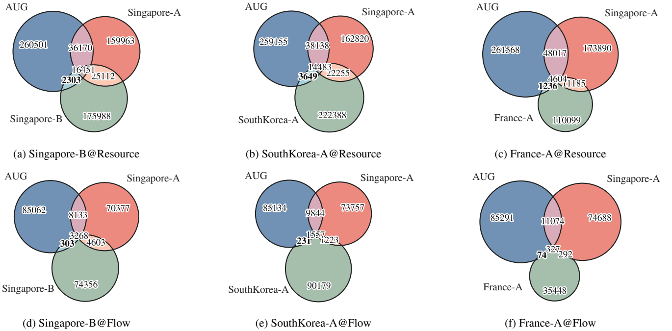
Fig. 9. Impact of frame sequence augmentation on pattern coverage at resource and flow granularities.
