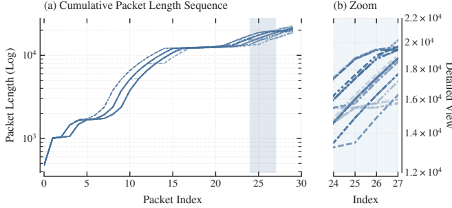
Fig. 4. Illustrative example of packet length sequence instability caused by HTTP/2 scheduling and cross-layer encapsulation.
