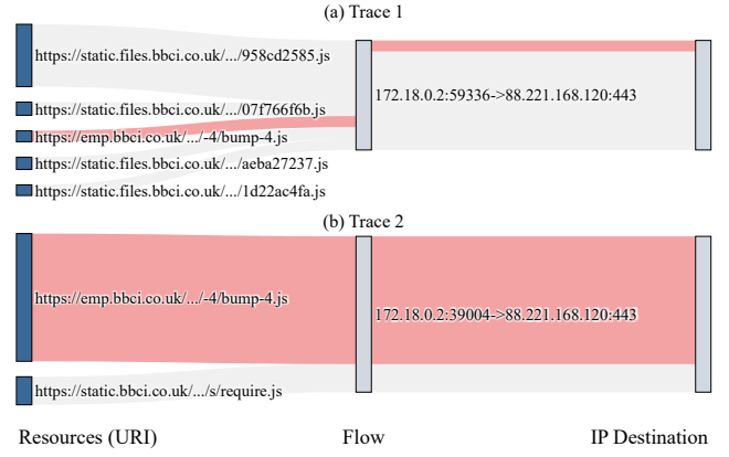
Fig. 2. Illustrative example of cross-domain resource aggregation caused by dynamic DNS and HTTP/2 connection coalescing.
