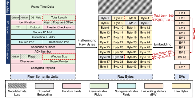
Figure 1. Protocol fields (left) are flattened into raw bytes (middle) and embedded (right), illustrating inductive bias mismatch at three levels: (P1) Field-level unpredictability: Random fields (pink) are treated as learnable despite being unpredictable by protocol design (e.g., ip.id and checksum ). (P2) Cross-field-level embedding confusion: Field distinctions are lost through cross-field embedding (grey), where adjacent bytes span multiple fields (e.g. ip.flags and ip.frag_offset ), and unified embedding function, where semantically different values receive identical vectors (e.g., Total Len=1500 and Win Size=1500 ). (P3) Flow-level metadata loss: Temporal metadata (hatched) essential for flow-level behavior analysis exists outside packet bytes and is entirely discarded.
