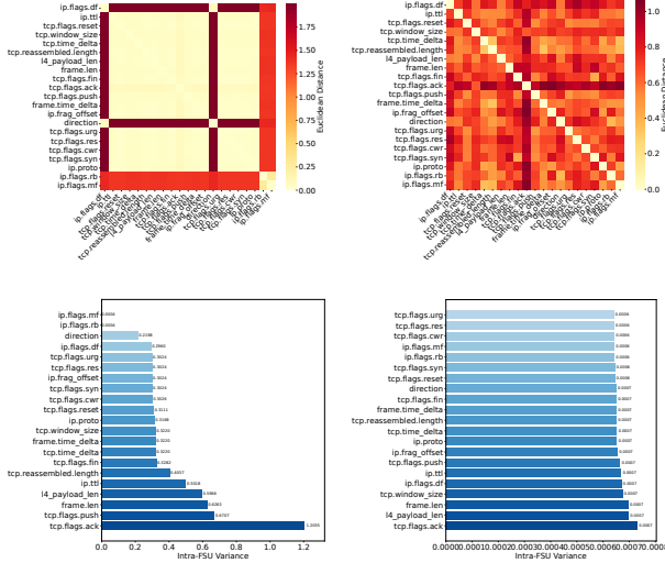
Figure 6. Embedding space analysis. Top: Inter-FSU centroid distances; Bottom: Intra-FSU variance. Left: Shared embeddings; Right: FSU-specific embeddings. FSU-specific embeddings achieve uniform separation (0.4–0.8) and consistent compactness ( \sim 0.0007 ), while shared embeddings show extreme distances (0–1.75) and 3000\times variance disparity.
