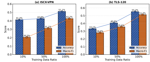
Figure 5. Performance under different labeled data ratios.
