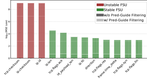
Figure 4. Effect of predictability-guided filtering on reconstruction loss. Without predictability-guided filtering, random fields (red) exhibit extremely high loss ( \sim 10^9 ) and degrade learning of generalizable fields (green).
