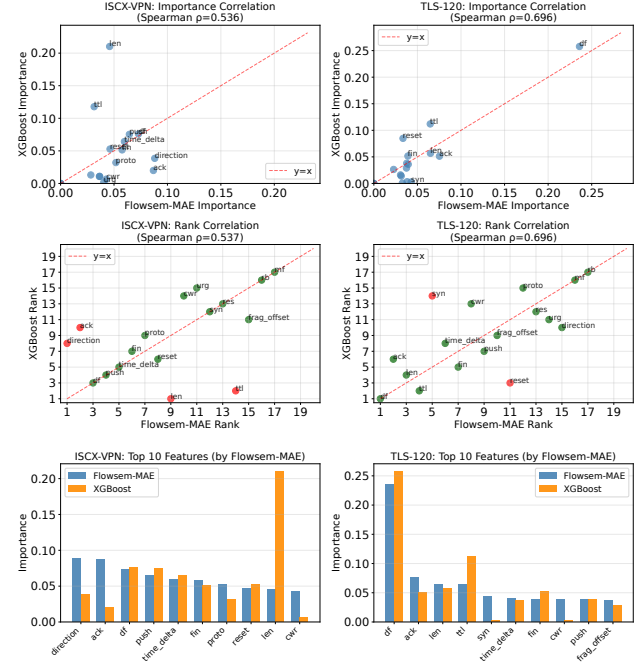
Figure 7. FSU importance comparing FlowSem-MAE with XGBoost. Moderate-to-strong Spearman correlation ( \rho = 0.536 on ISCX-VPN, \rho = 0.696 on TLS-120) indicates FlowSem-MAE discovers similar discriminative features while capturing additional interaction patterns.
