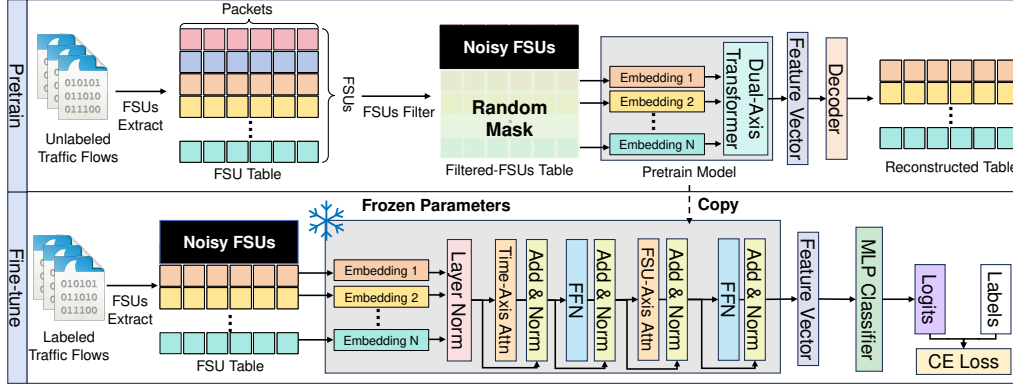
Figure 2. Workflow of FlowSem-MAE. Noisy FSUs refer to the union of random and non-generalizable fields.
