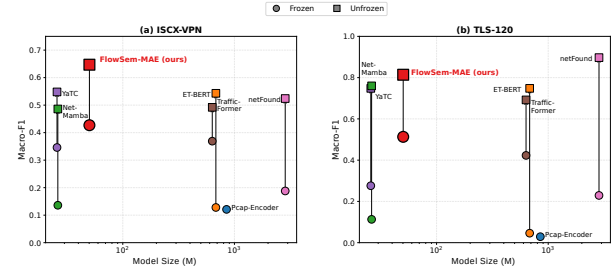
Figure 3. Model size vs. performance (Macro-F1). FlowSem-MAE achieves the best performance with only 50.25M model size, significantly outperforming larger models.
