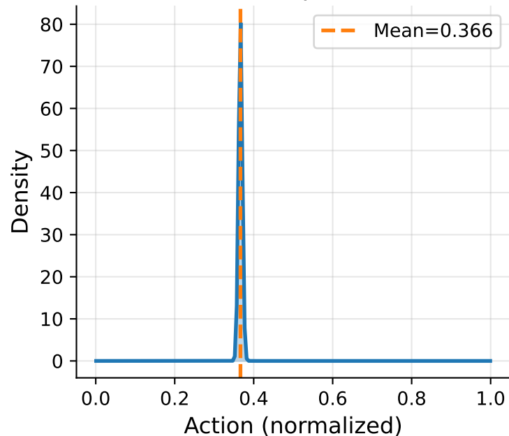
Step 204800 (10%) \alpha=3512.3 , \beta=6072.2
