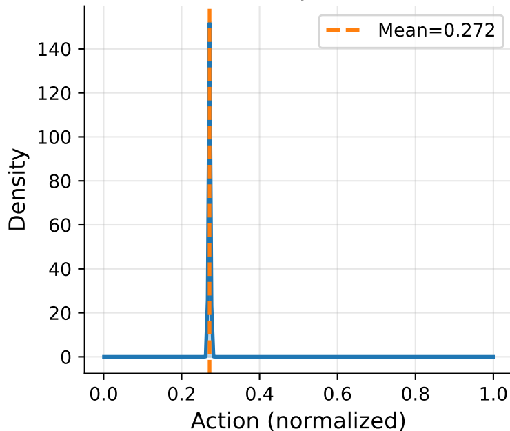
Step 1019904 (50%) \alpha=7805.5 , \beta=20918.8
