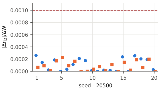
|\text{stage-1 error}| (S1, secondary)
