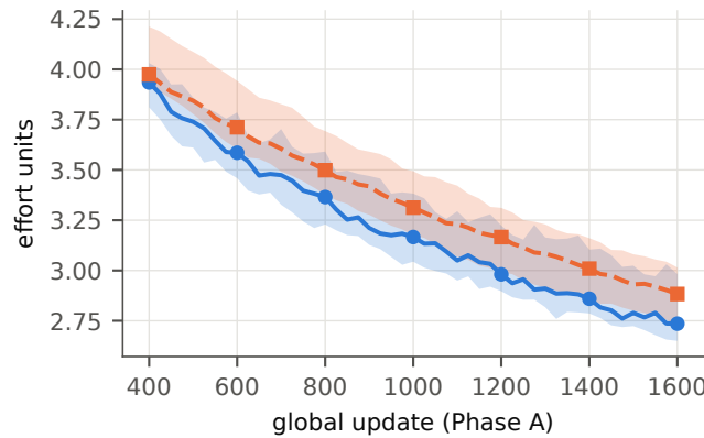
\sigma_z(0)
