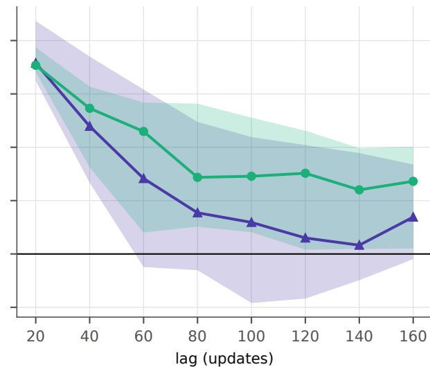
q = 60, ACF about e_{1*} (not demeaned)
