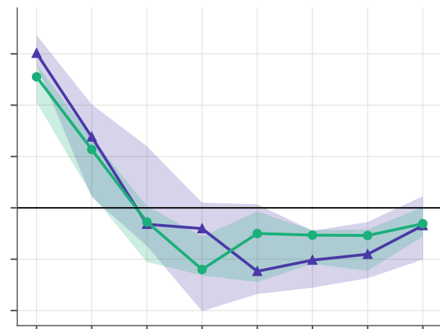
q = 60, ACF about e_{1*} (not demeaned)
