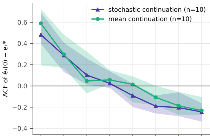
q = 50, ACF about e_{1*} (not demeaned)
