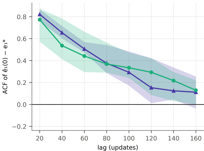
q = 50, ACF about e_{1*} (not demeaned)
