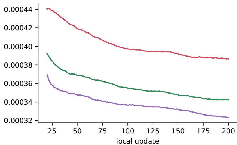
q = 60: logged FOC residual (rolling mean 20)
