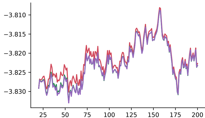
q = 60: logged FOC residual (rolling mean 20)
