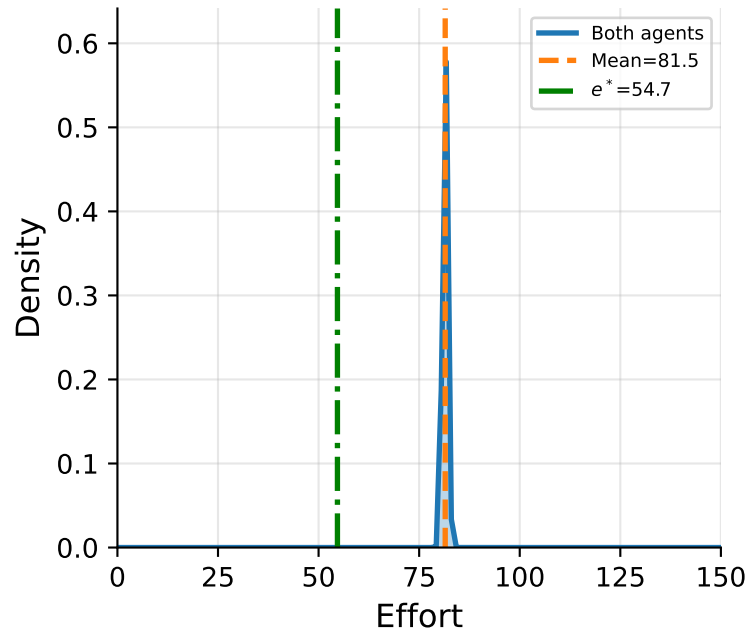
Step 2576384 (50%)
