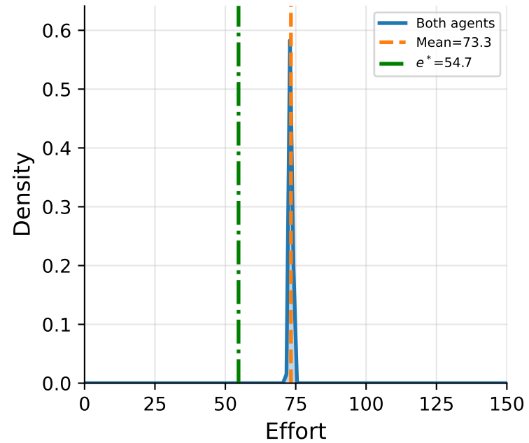
Step 4636672 (90%)
