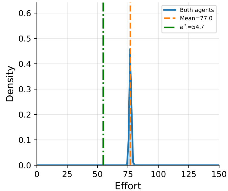
Step 516096 (10%)
