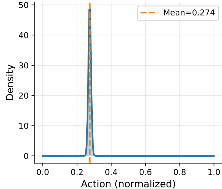
Step 131072 (10%) \alpha=896.0 , \beta=2368.7
