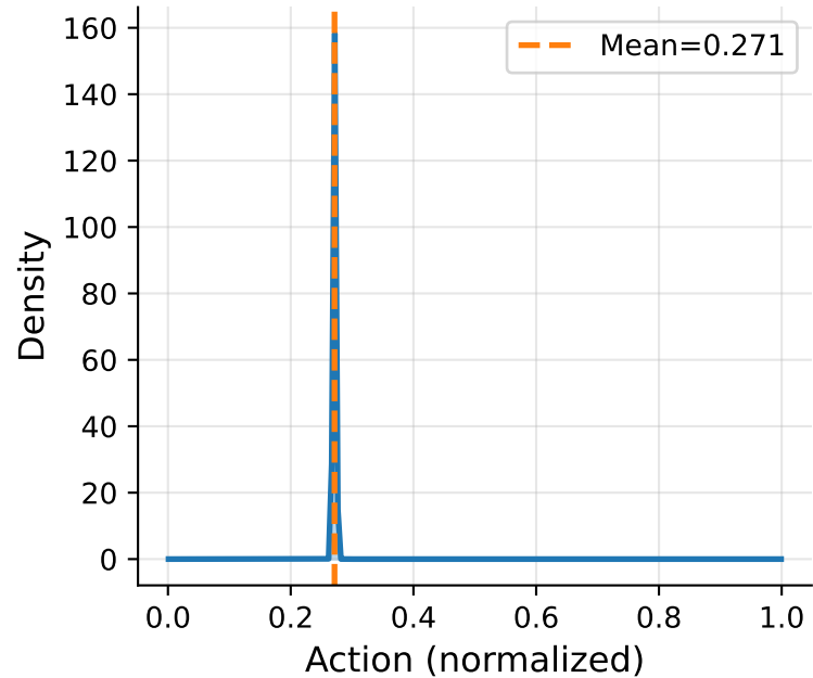
Step 1306624 (100%) \alpha=8694.1 , \beta=23339.5
