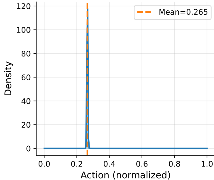
Step 651264 (50%) \alpha=6537.8 , \beta=18124.7
