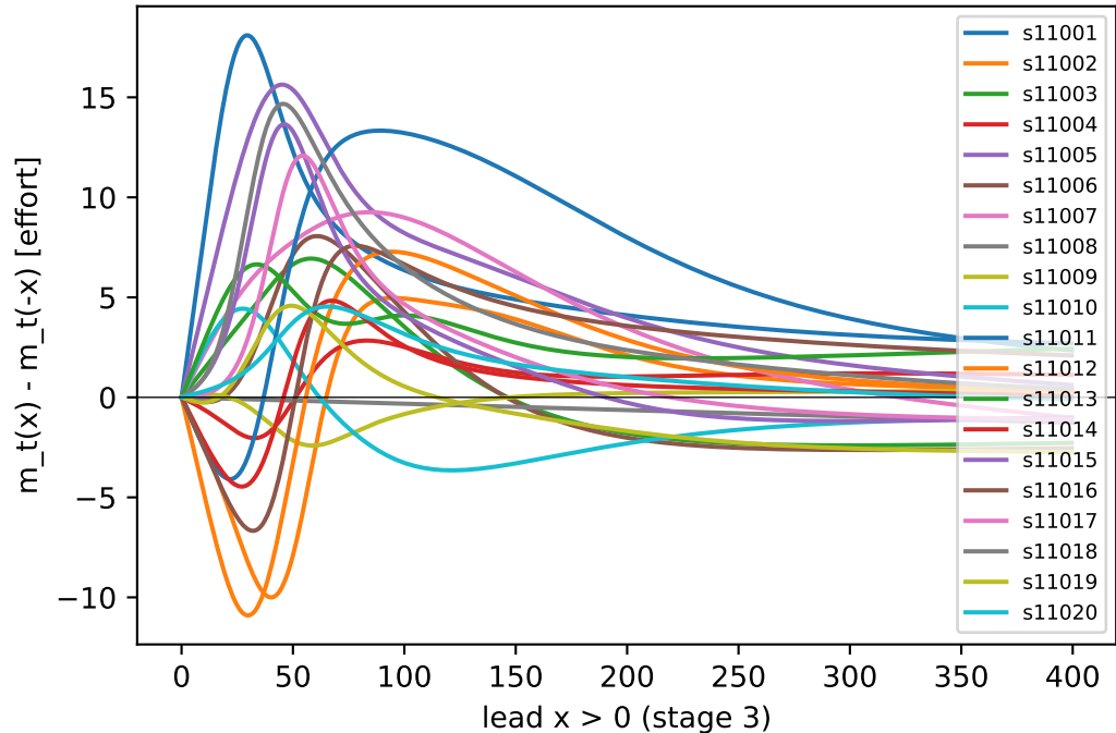
q=50, stage 3: leader - follower policy
