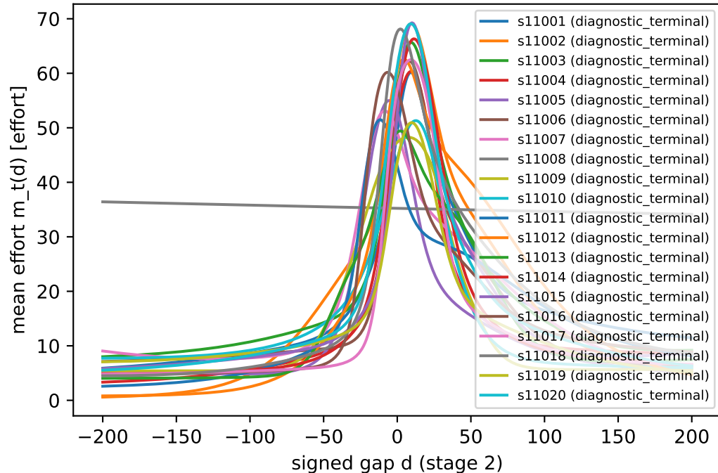
q=50, stage 2: endpoint mean policy
