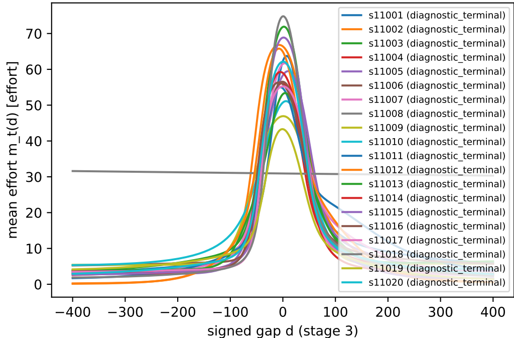
q=50, stage 3: endpoint mean policy
