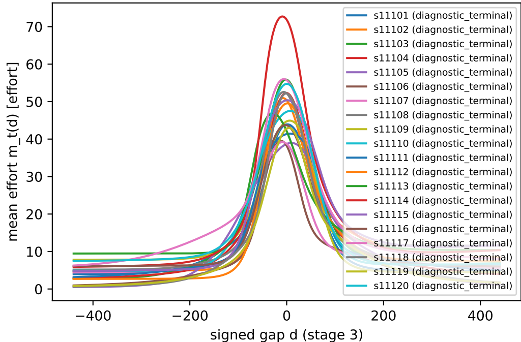
q=60, stage 3: endpoint mean policy
