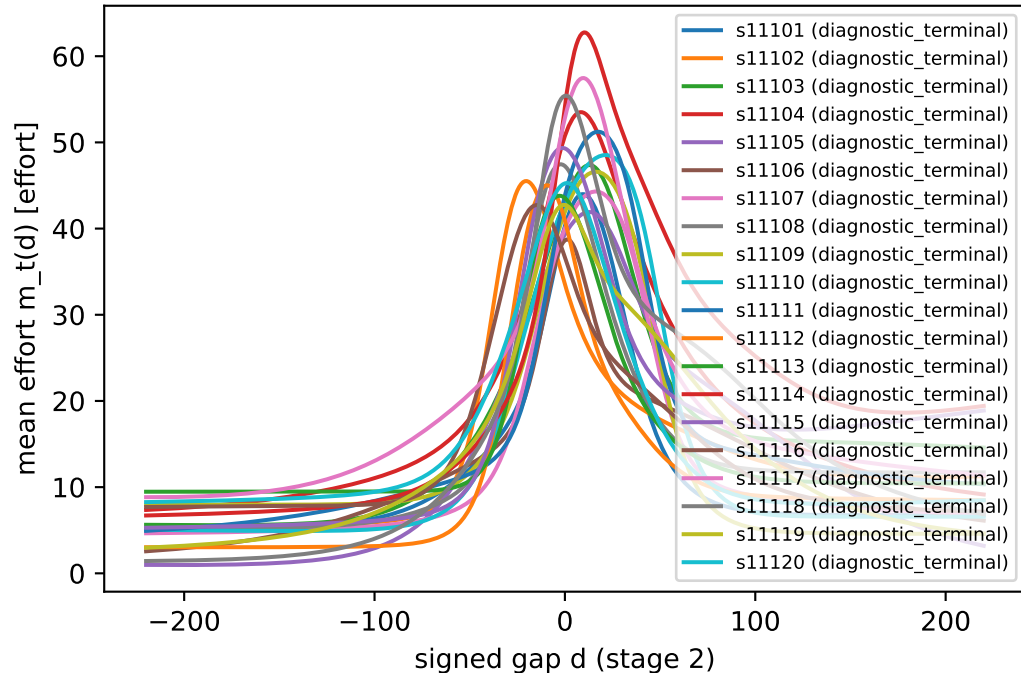
q=60, stage 2: endpoint mean policy
