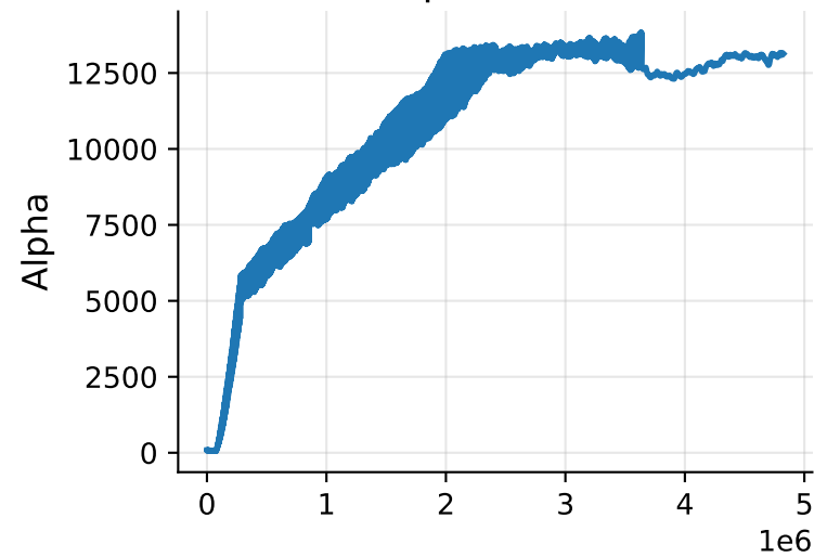
q = 35.0
