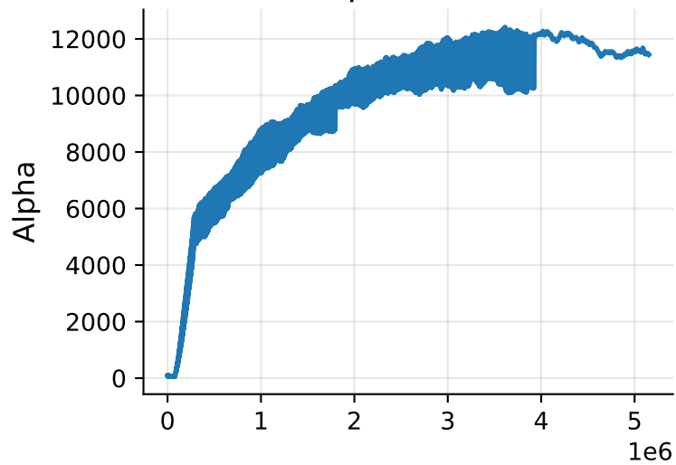
q = 40.0
