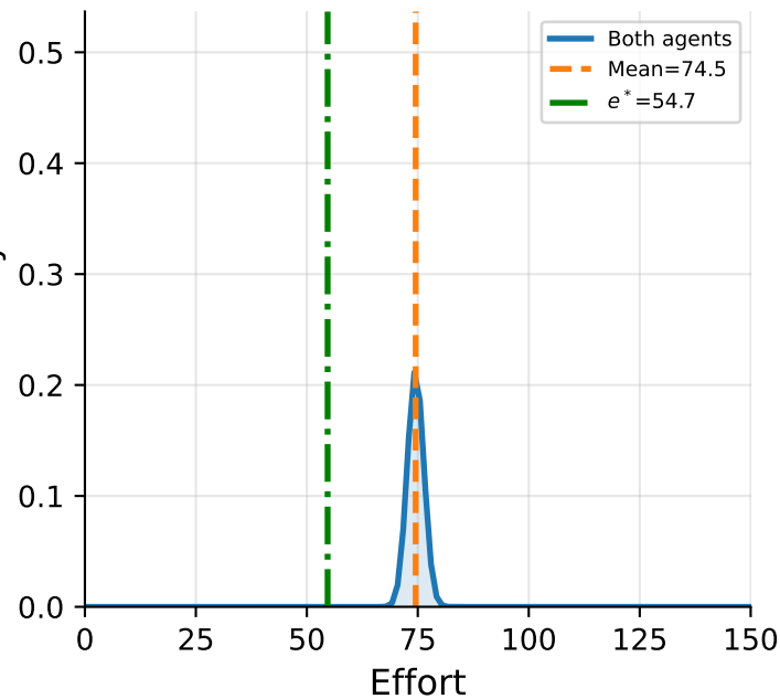
Step 131072 (10%)
