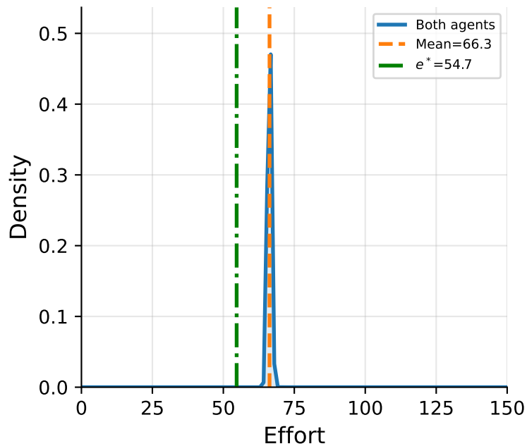
Step 651264 (50%)
