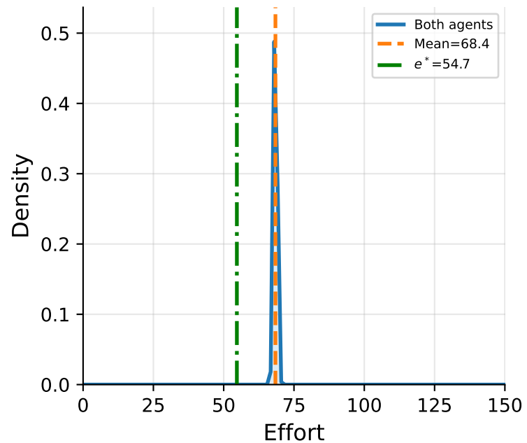
Step 1175552 (90%)
