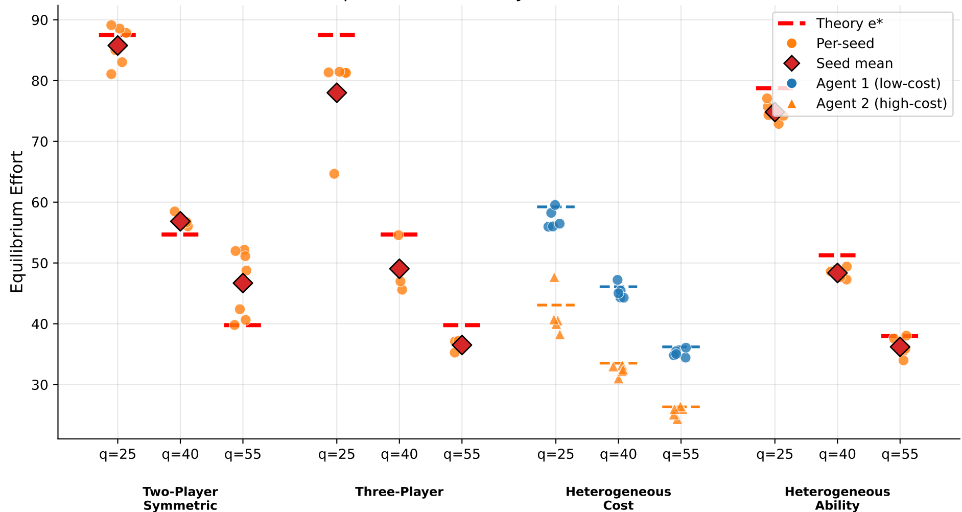
Equilibrium Recovery Across Scenarios
